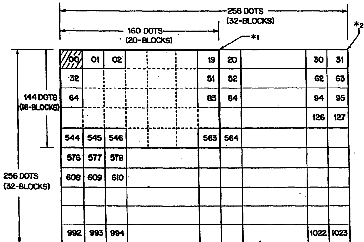
FIG. 14 BACKGROUND (BG) DISPLAY
