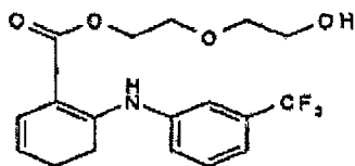
etofenamate
