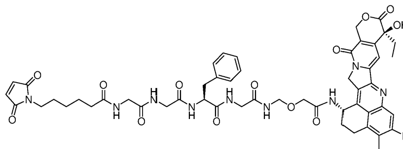
MC-GGFG-DXD
