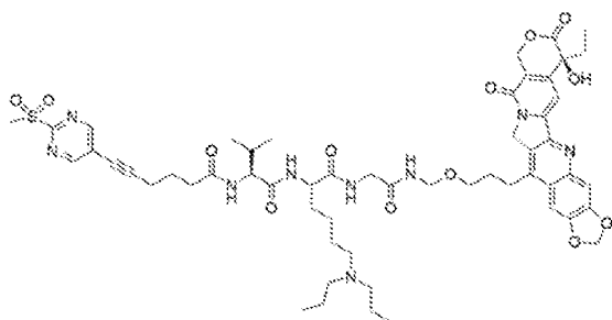
LP62
