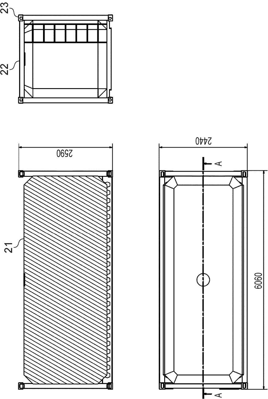
Generic 20' ISO Container frame with CRY-Fuel vacuum insulated tank
