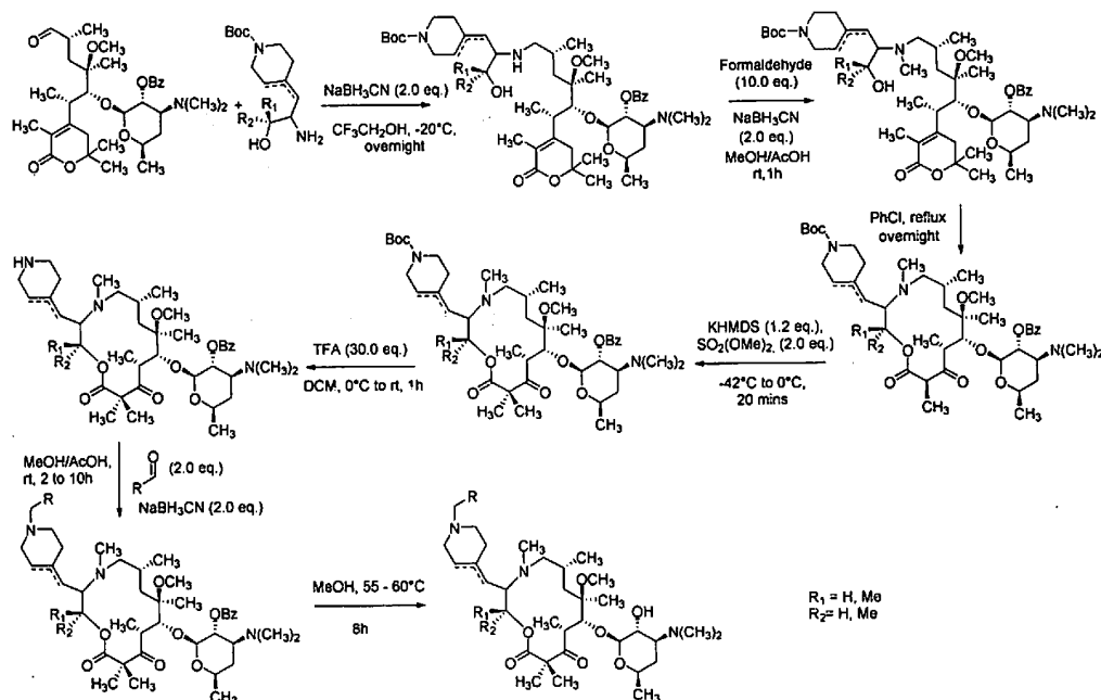
Scheme 7.
