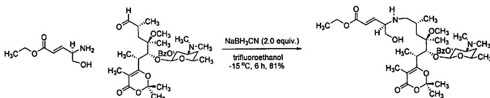
Scheme 9.
