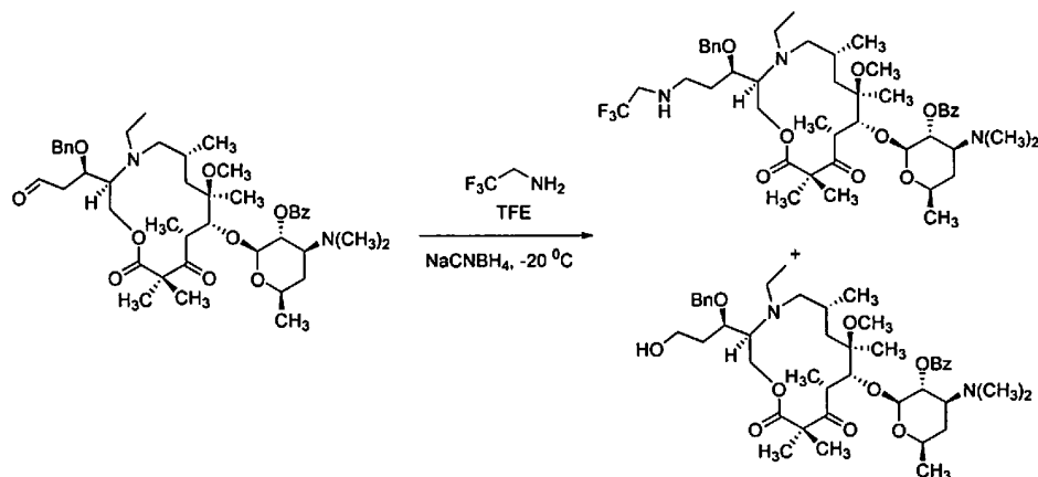
Scheme 12.
