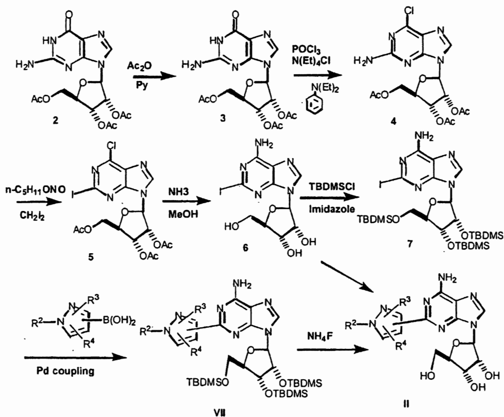
Scheme 3
