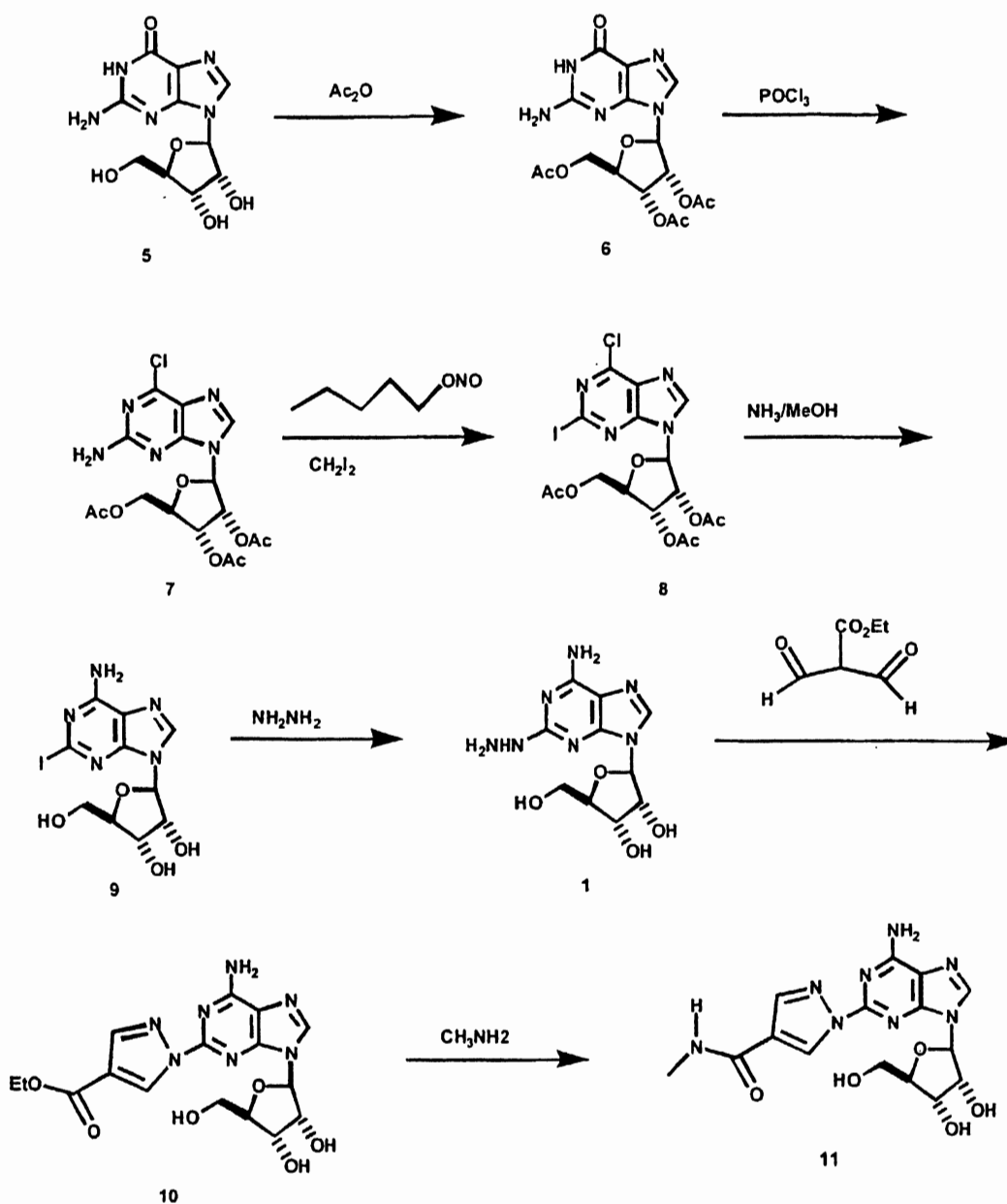
Scheme 3
