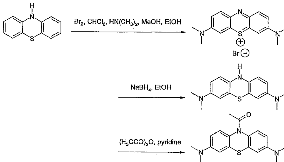
Scheme 6
