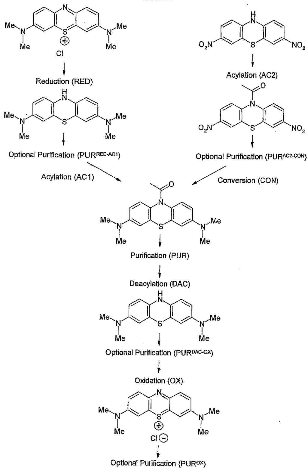
Scheme 9
