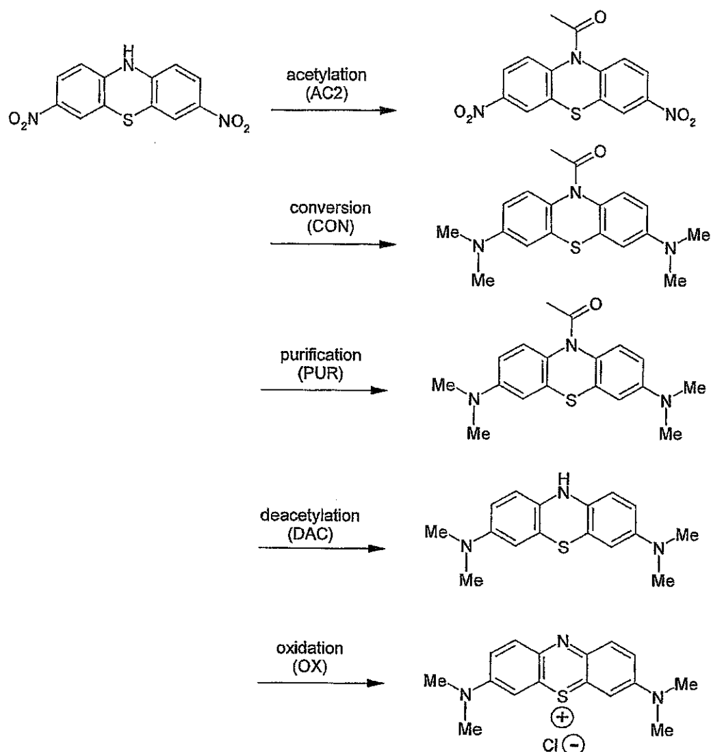
Scheme 20
