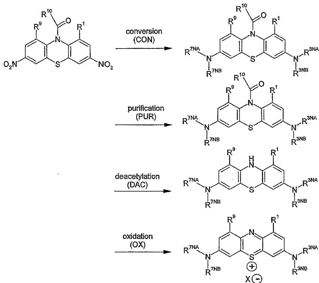
Scheme 17
