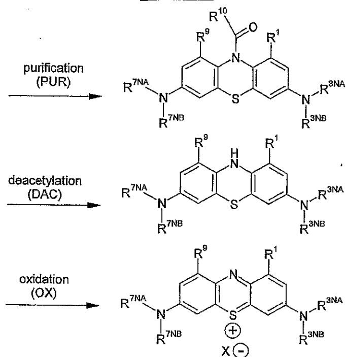
Scheme 10
