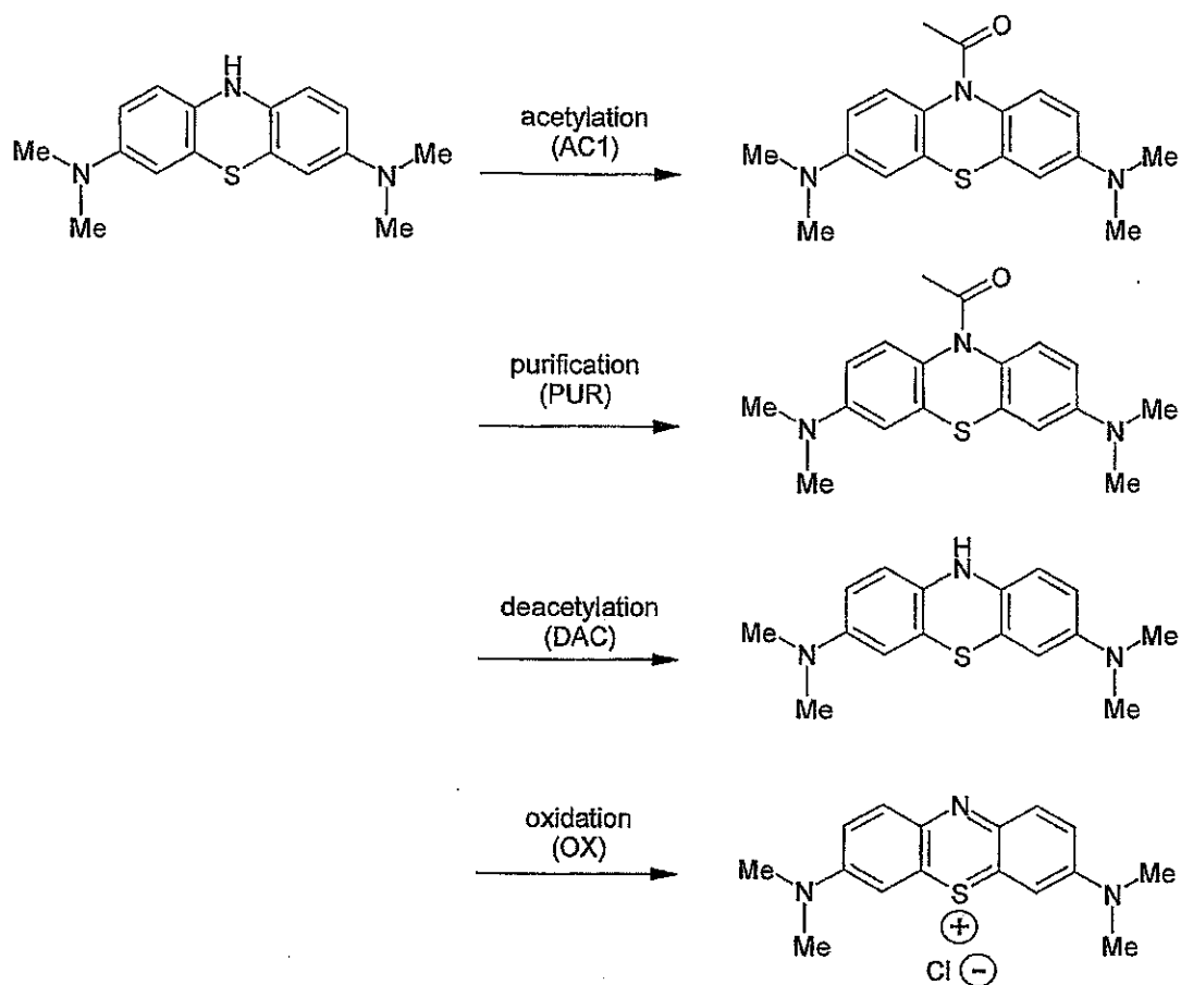
Scheme 13
