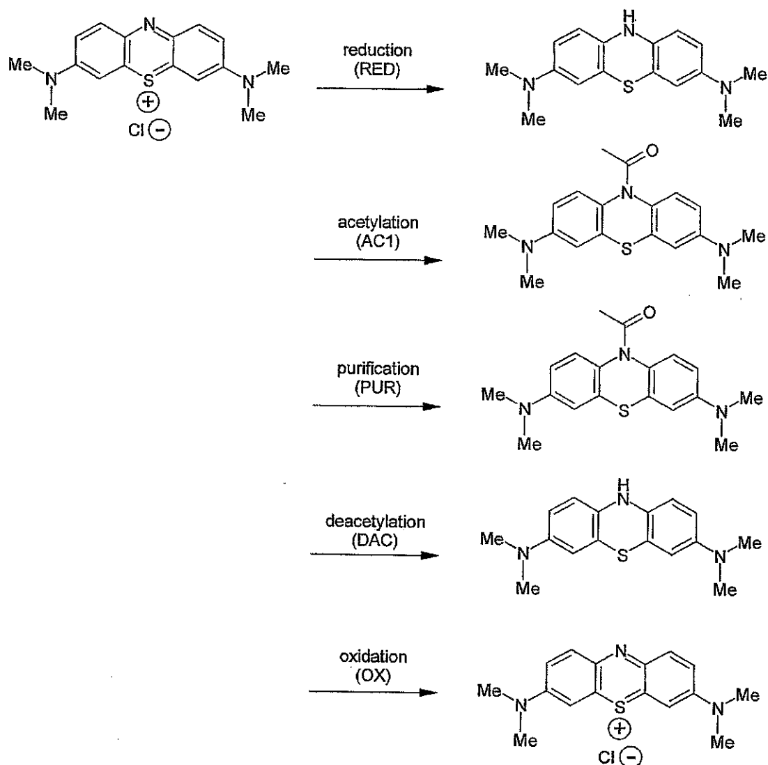
Scheme 15
