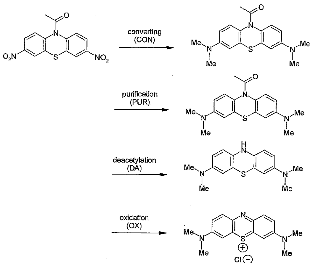
Scheme 18
