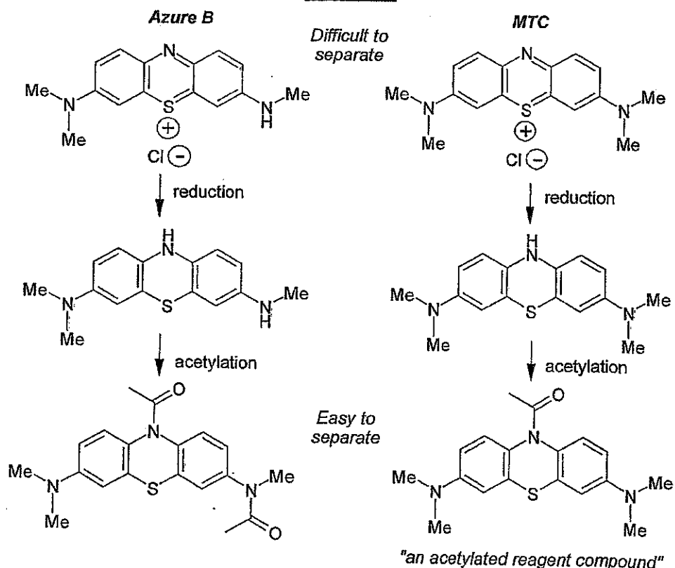
Scheme 8
