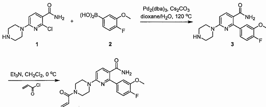
Example 30
