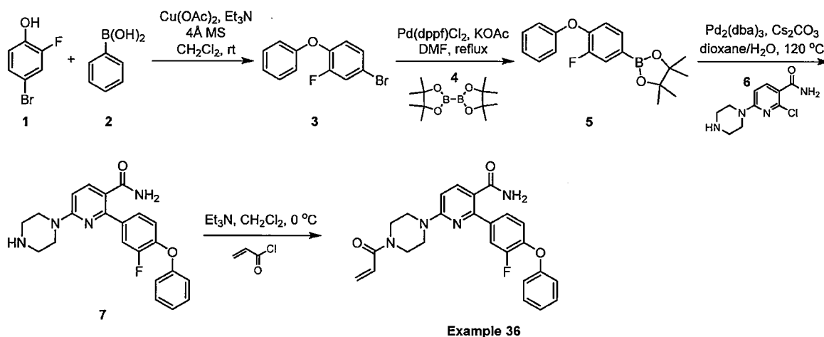
Example 36
