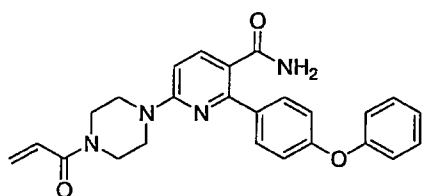
6-(4-acryloylpiperazin-1-yl)-2-(4-phenoxyphenyl)nicotinamide;
