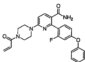
6-(4-acryloylpiperazin-1-yl)-2-(2-fluoro-4-phenoxyphenyl)nicotinamide.
