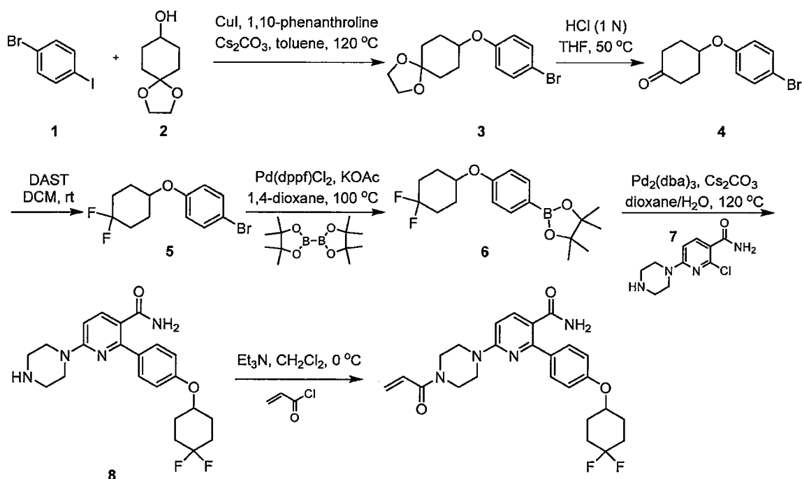
Example 60
