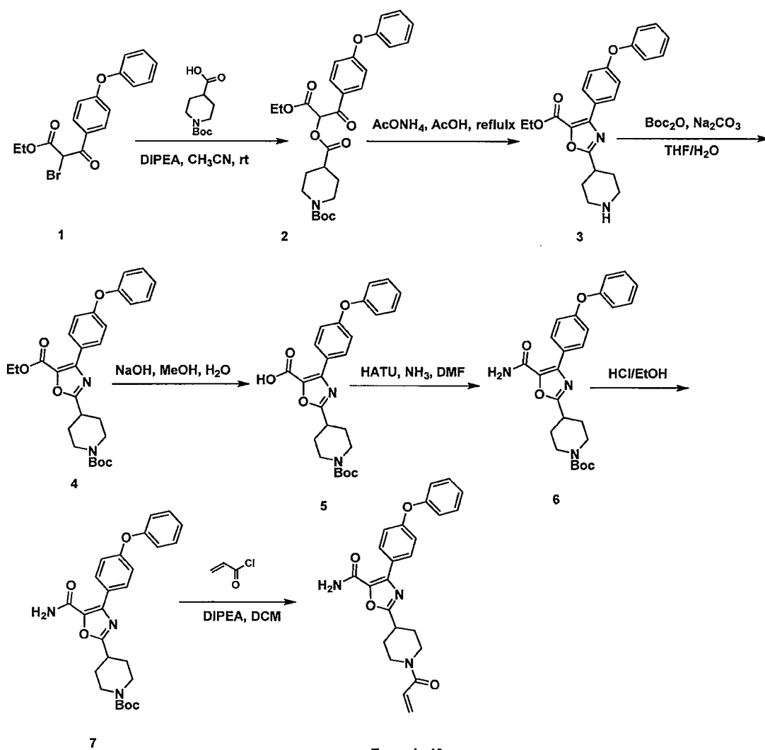
Example 46
