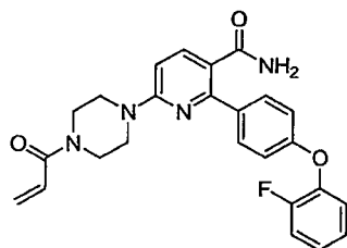
6-(4-acryloylpiperazin-1-yl)-2-(4-(2-fluorophenoxy)phenyl)nicotinamide
