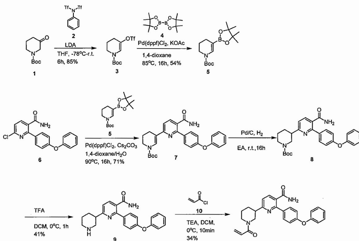
Example 8
