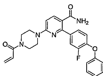
6-(4-acryloylpiperazin-1-yl)-2-(3-fluoro-4-phenoxyphenyl)nicotinamide
