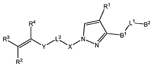
Ib
