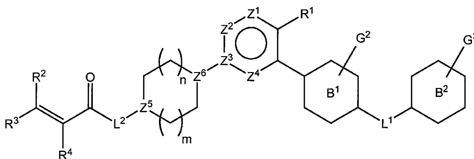
IIId
