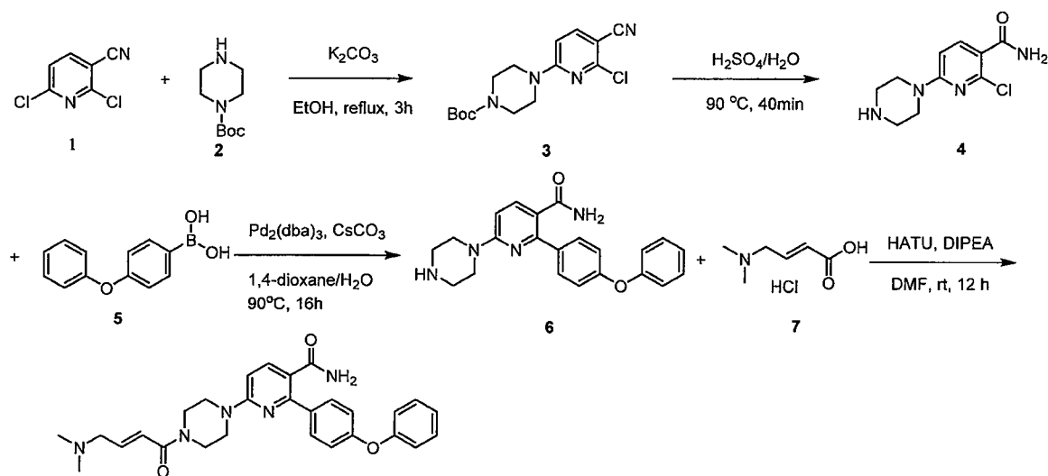
Example 25
