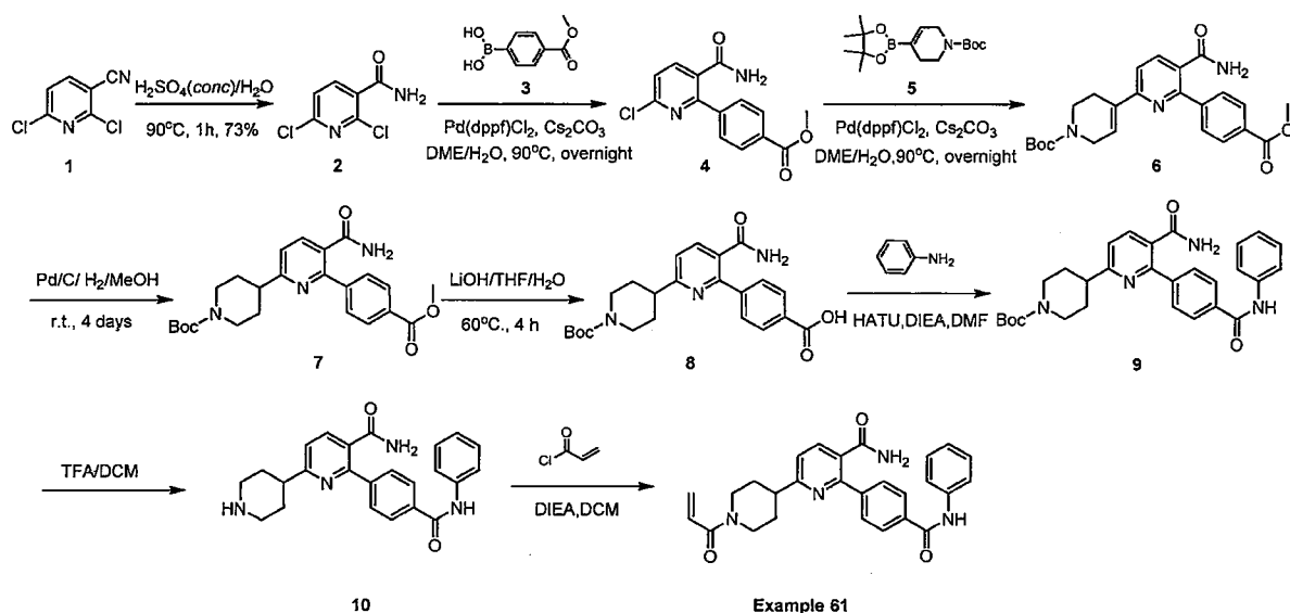
Example 61
