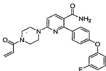
6-(4-acryloylpiperazin-1-yl)-2-(4-(3-fluorophenoxy)phenyl)nicotinamide
