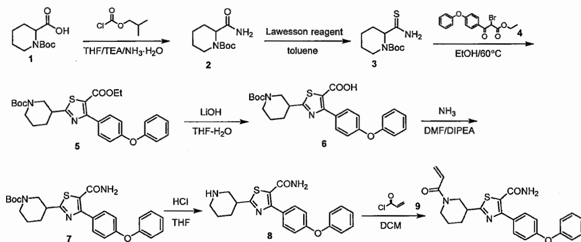
Example 40
