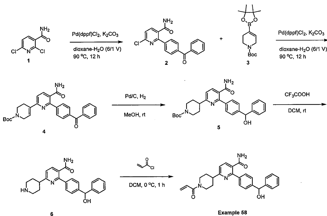
Example 58
