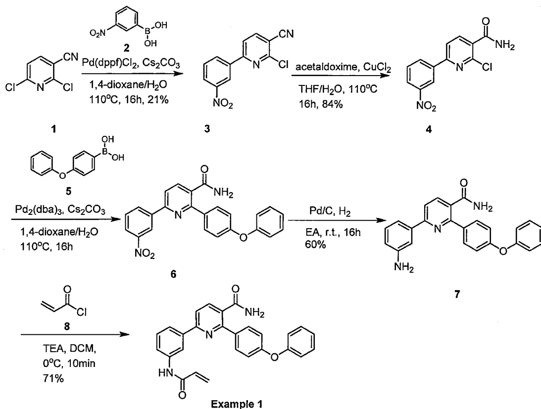
Example 1
