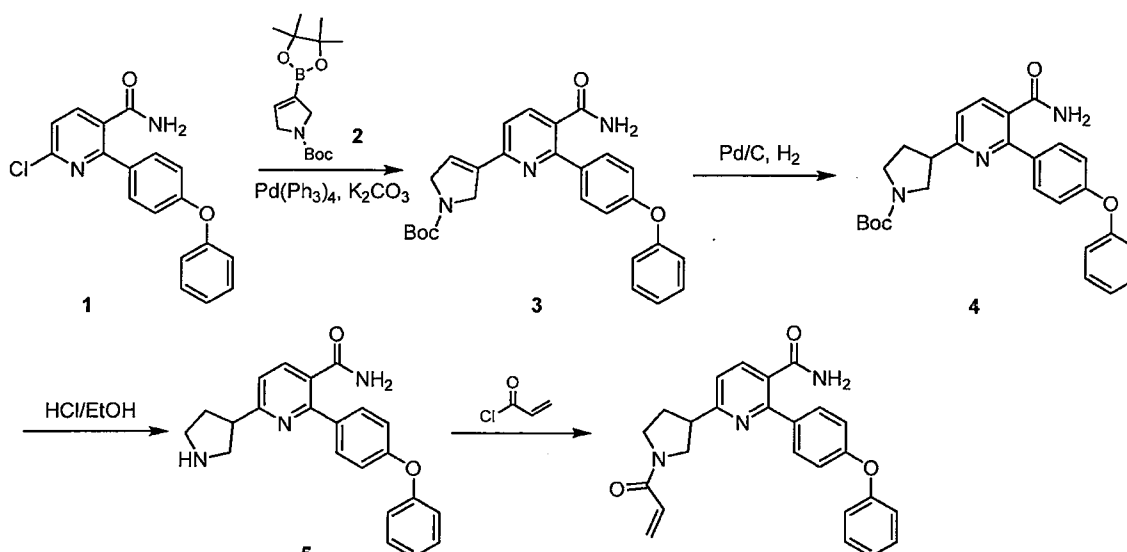
Example 6
