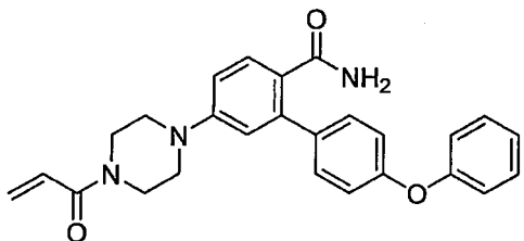
5-(4-acryloylpiperazin-1-yl)-4'-phenoxybiphenyl-2-carboxamide.
