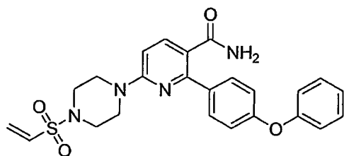
2-(4-phenoxyphenyl)-6-(4-(vinylsulfonyl)piperazin-1-yl)nicotinamide
