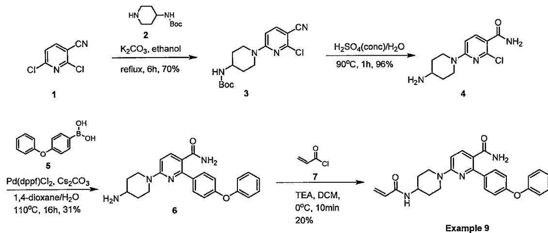
Example 9
