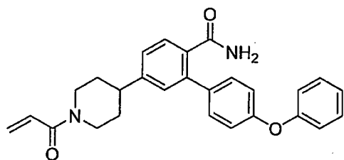
5-(1-acryloylpiperidin-4-yl)-4'-phenoxybiphenyl-2-carboxamide
