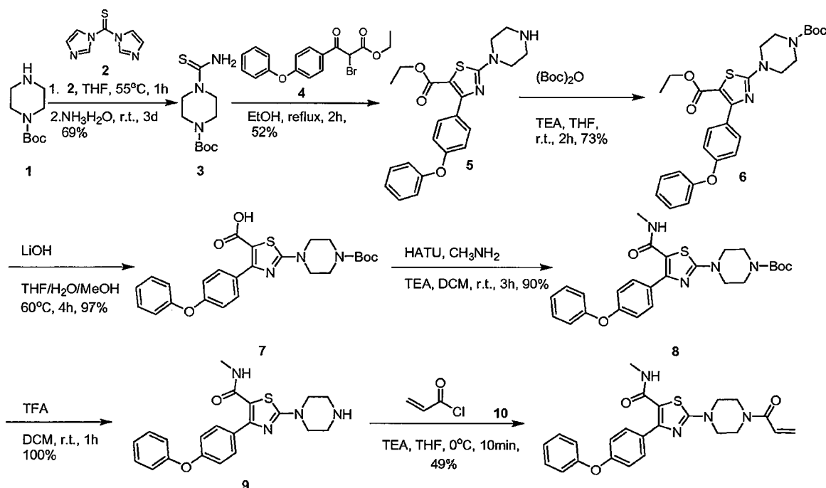
Example 47
