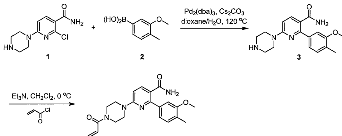
Example 29
