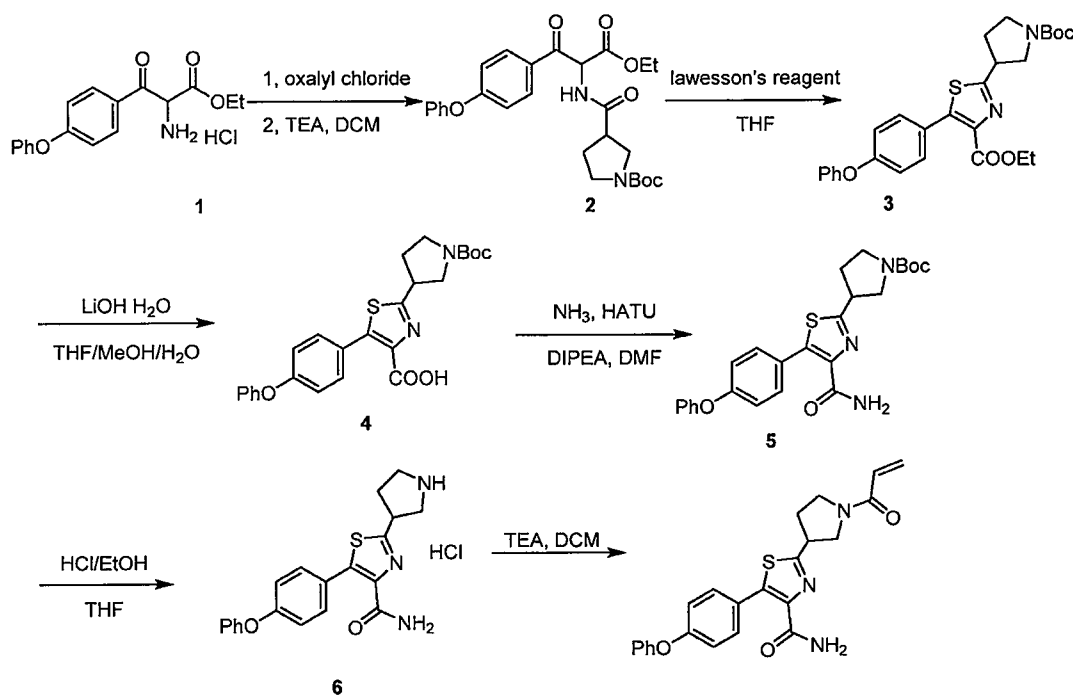
Example 44
