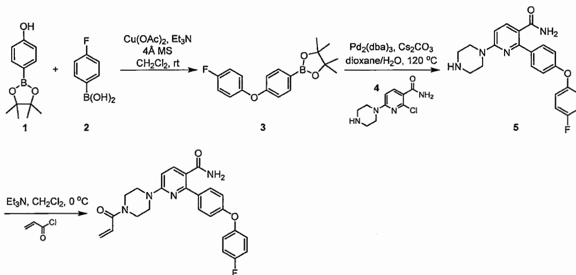
Example 37
