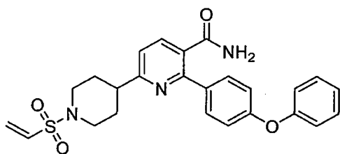
2-(4-phenoxyphenyl)-6-(1-(vinylsulfonyl)piperidin-4-yl)nicotinamide.
