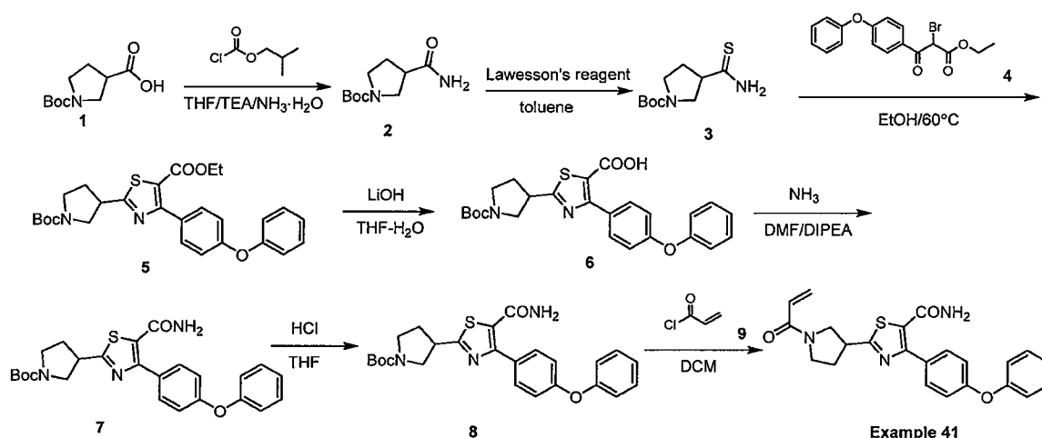
Example 41
