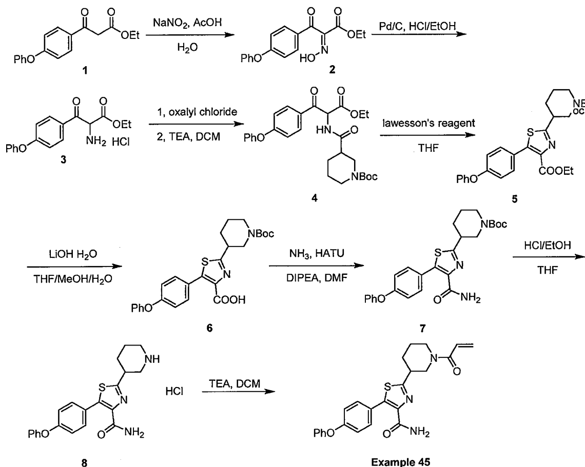
Example 45
