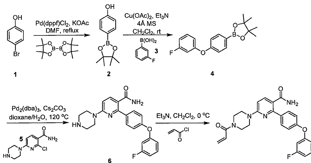
Example 35
