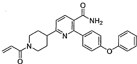
6-(1-acryloylpiperidin-4-yl)-2-(4-phenoxyphenyl)nicotinamide.
