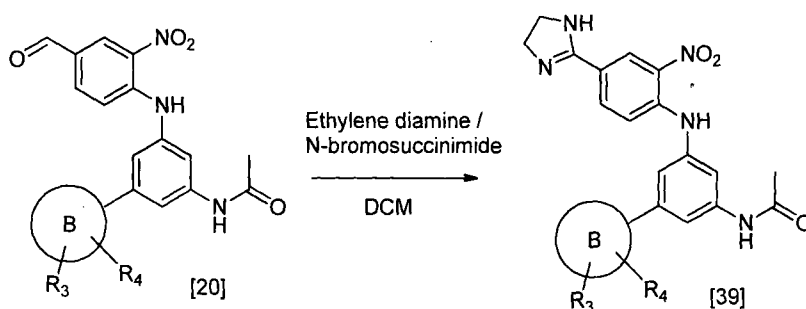
SCHEME 9.
