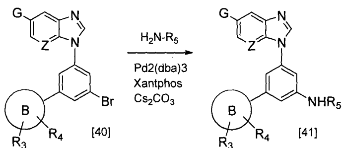
SCHEME 13.
