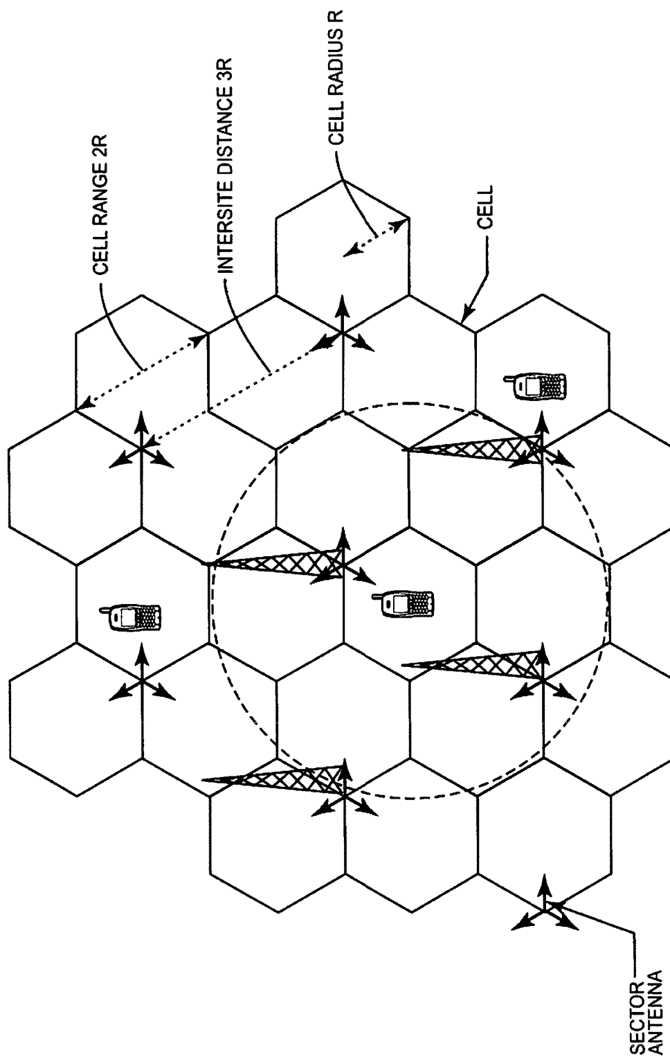
FIG. 5 (PRIOR ART)
