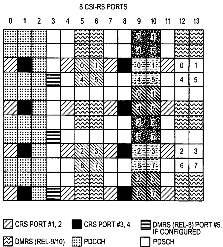
FIG. 8C (PRIOR ART)
