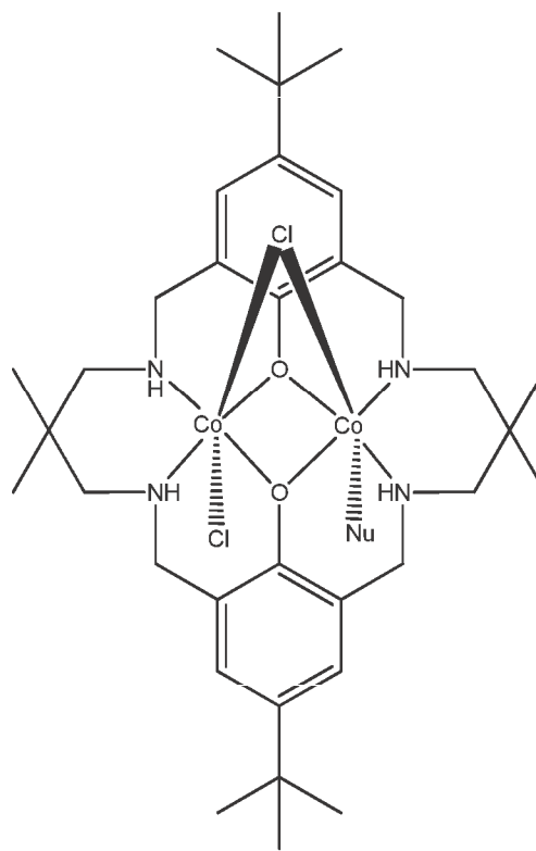
[L^1Co_2Cl_2Nu]
