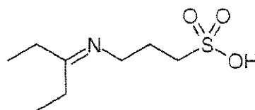
Compound M2
