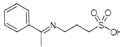
Compound M6
