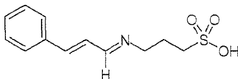
Compound M5
