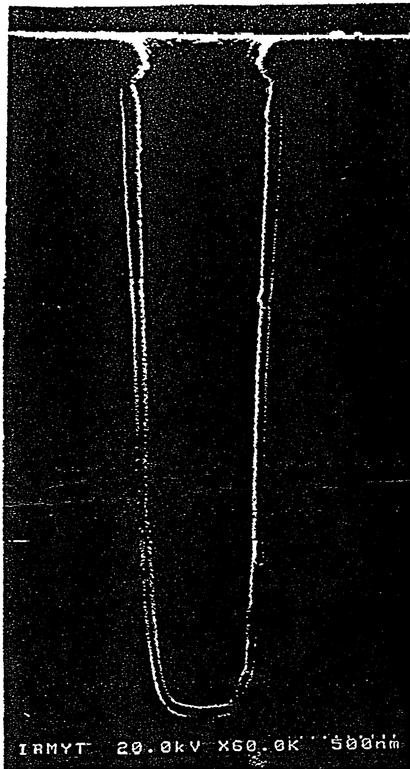
SEM of liner applied by collimated sputtering prior to CVD of Tungsten
