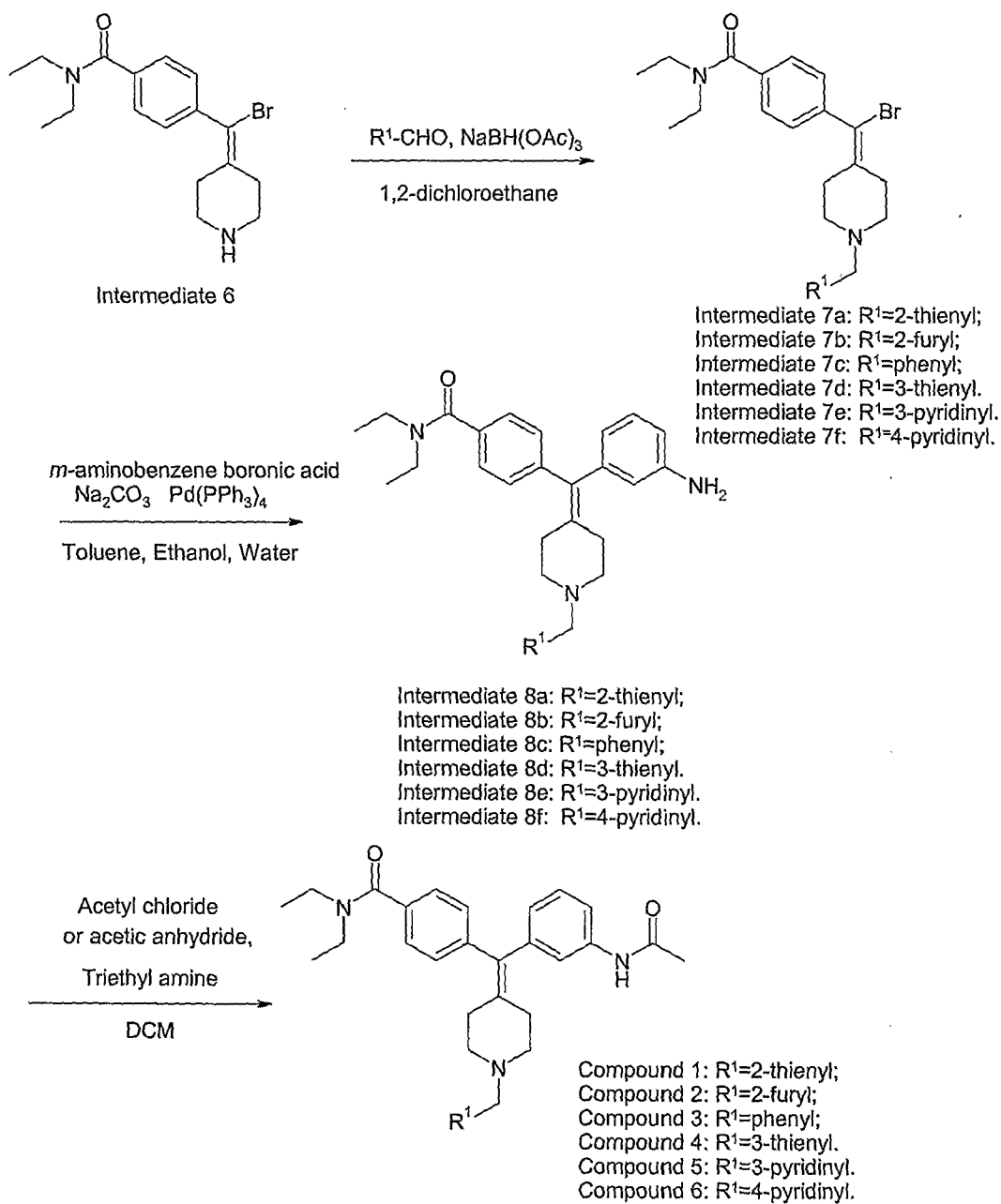
Scheme 2
