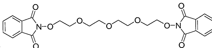
Synthesis of
