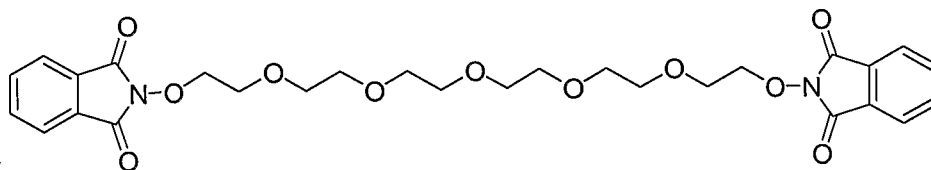
Synthesis of
