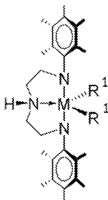
Formula III.
