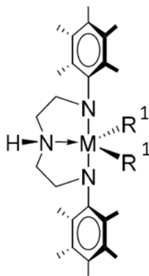
Formula III
