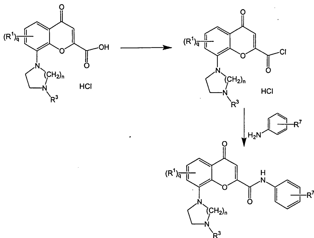
Scheme 2. Amide synthesis via acid chloride intermediate, wherein R^1 , R^3 , R^7 , n and q are as defined in the specification.
