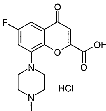
6-Fluoro-8-(4-methyl-piperazin-1-yl)-4-oxo-4H-chromene-2-carboxylic acid hydrochloride.
