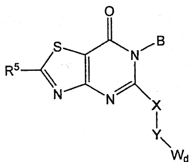
Formula XI
