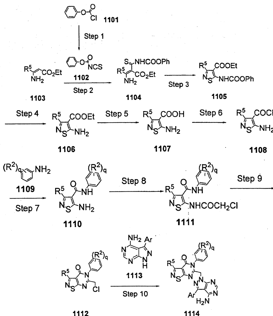
Reaction Scheme 11:
