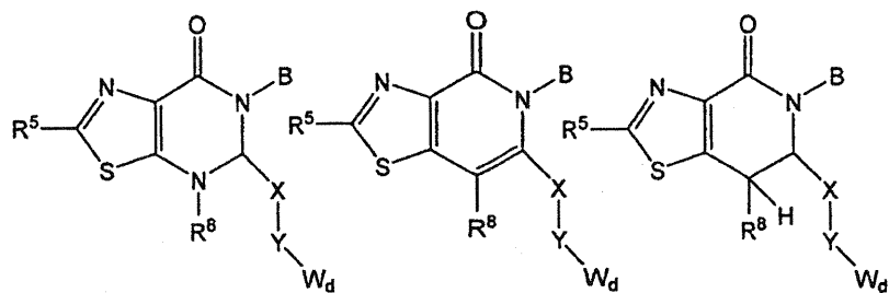
Formula 9-AB
