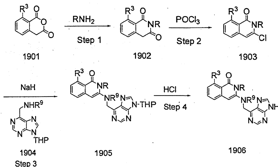
Reaction Scheme 19:
