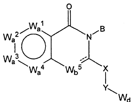
Formula I
