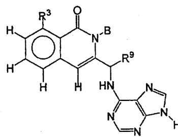
Formula 6-C1
