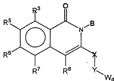
Formula VI
