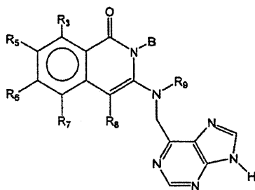
Formula VI-D
