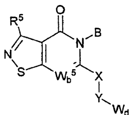
Formula XII
