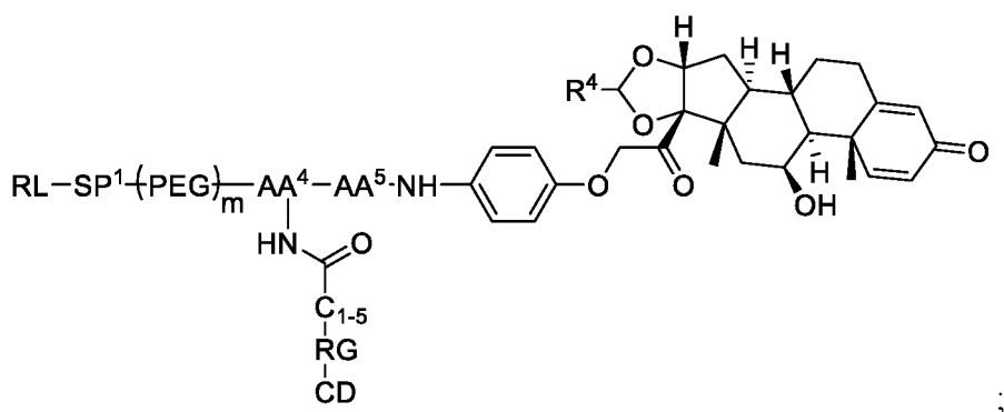
Formula ( IIIc-R )
