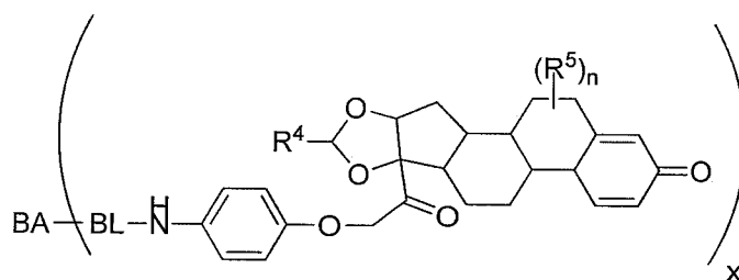
(IIIb);
