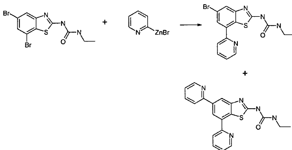
Scheme 10
