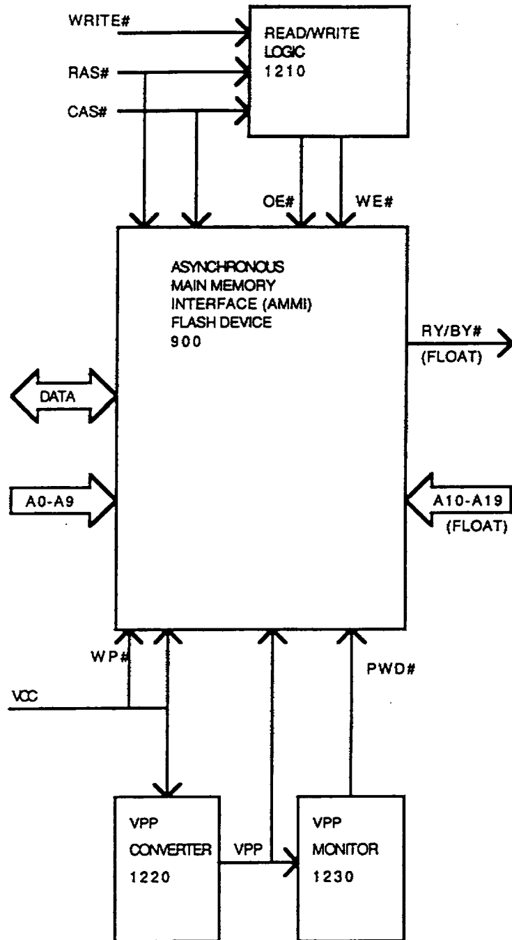
AMMI SINGLE IN-LINE MEMORY MODULE (SIMM) 1200
