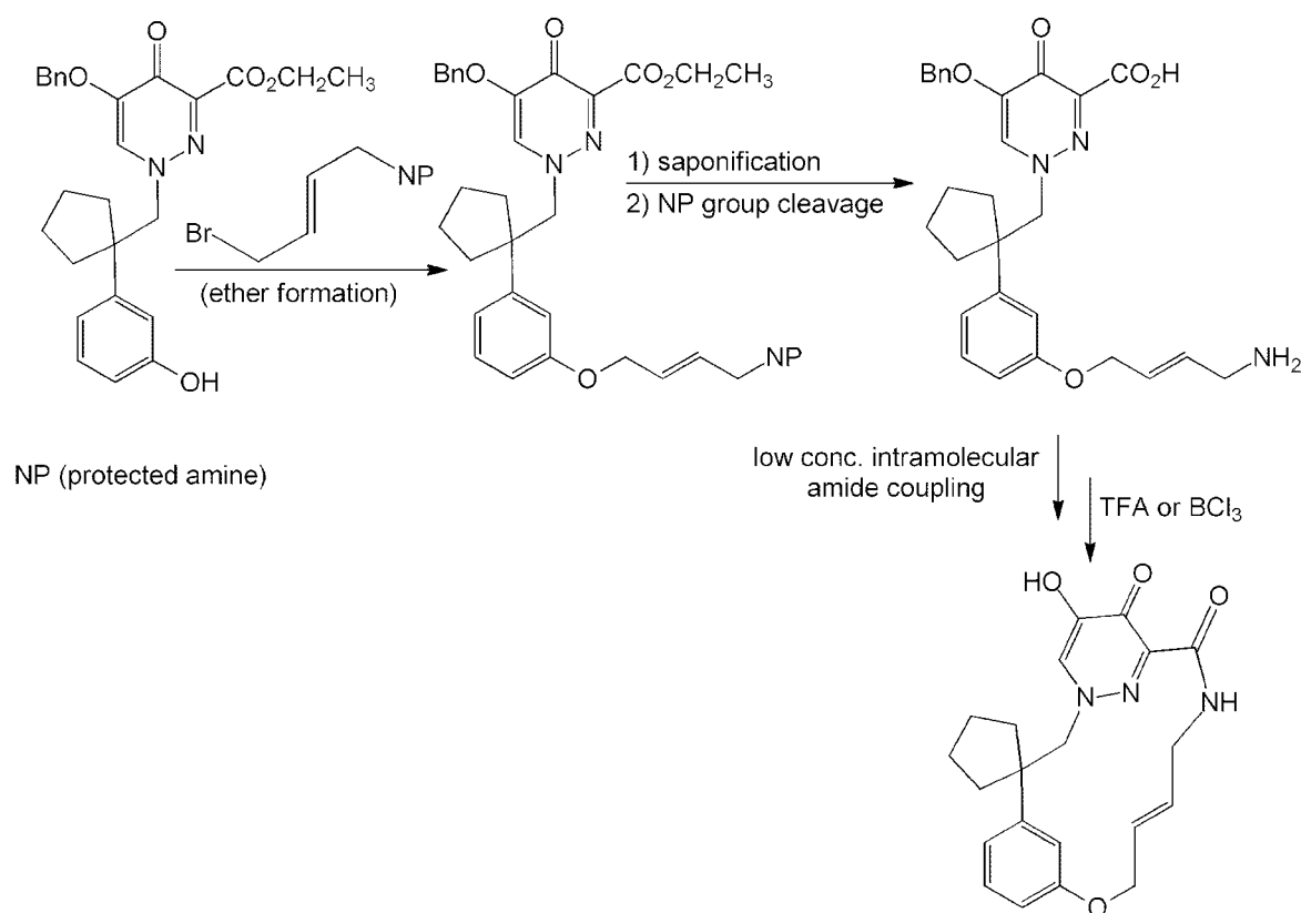
Scheme 10
