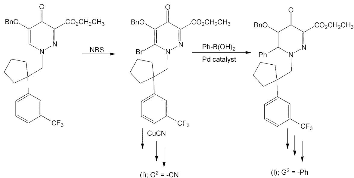
Scheme 8
