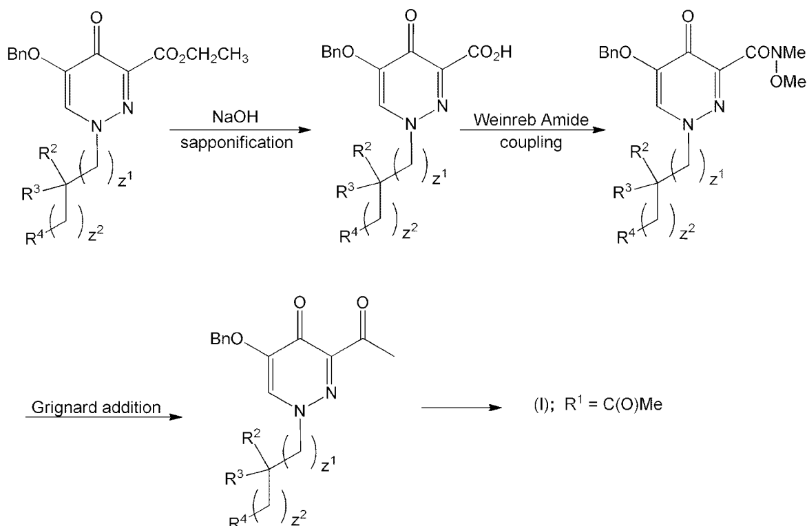
Scheme 6
