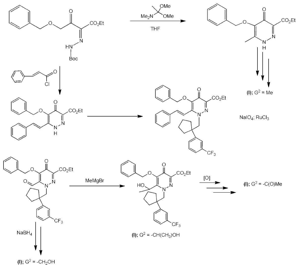
Scheme 7
