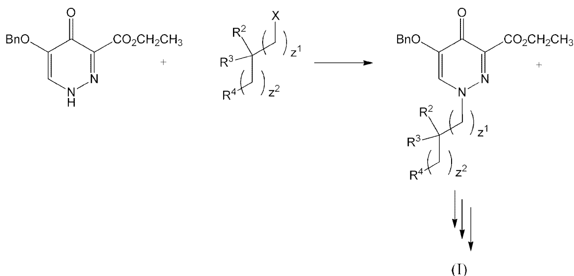
Scheme 4
