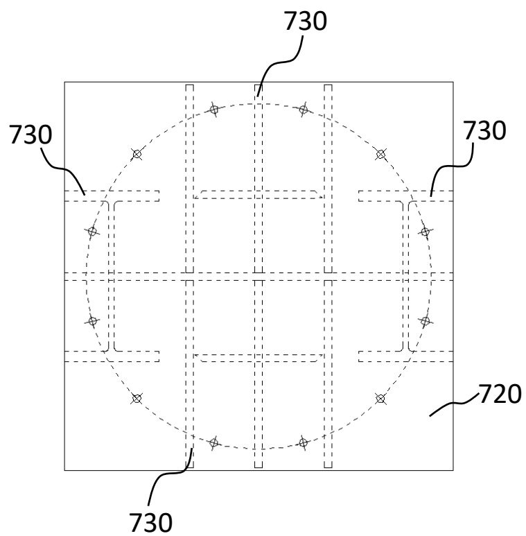
FIG. 45 (VIEW D4-D4)
