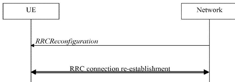
B : RRC reconfiguration, failure
