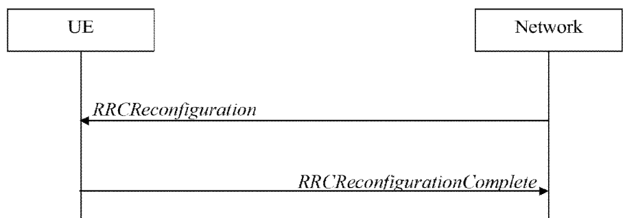
A : RRC reconfiguration, successful
