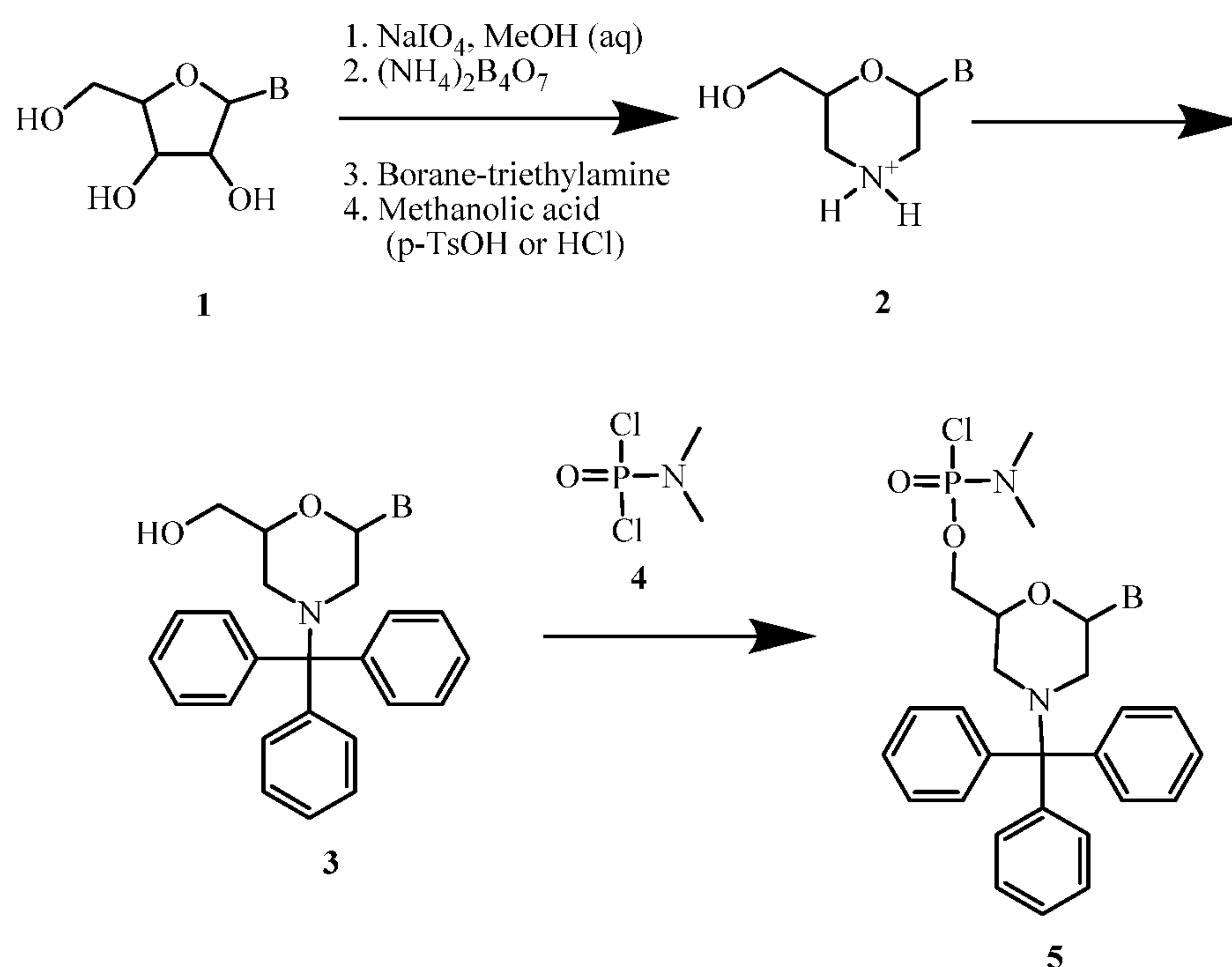
Scheme 1: General synthetic route to PMO Subunits
