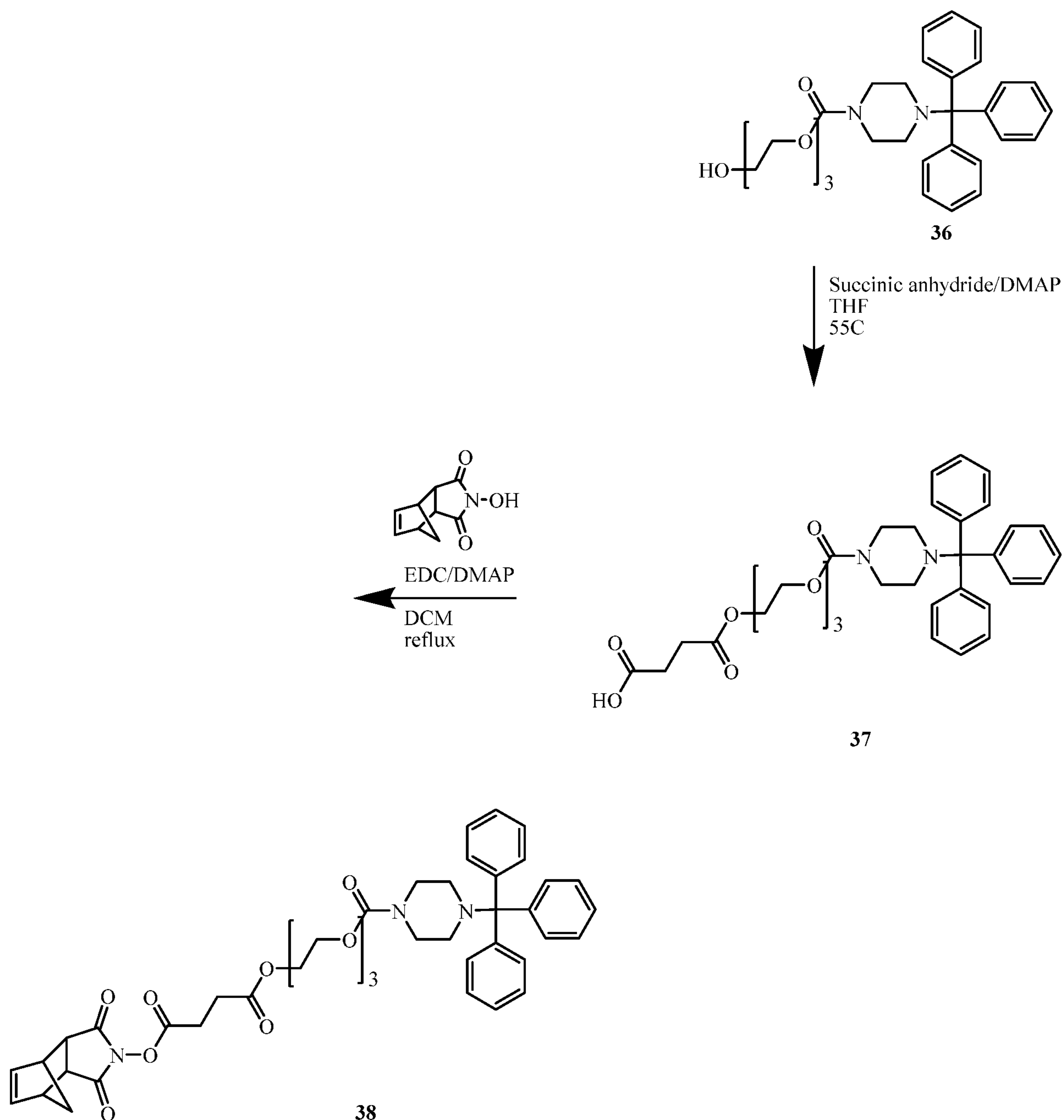
Scheme 2: Preparation of Activated Tail Acid
