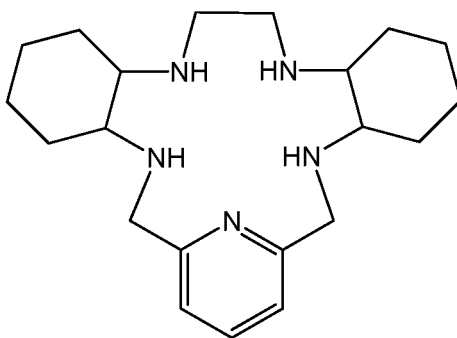
FORMULA B
