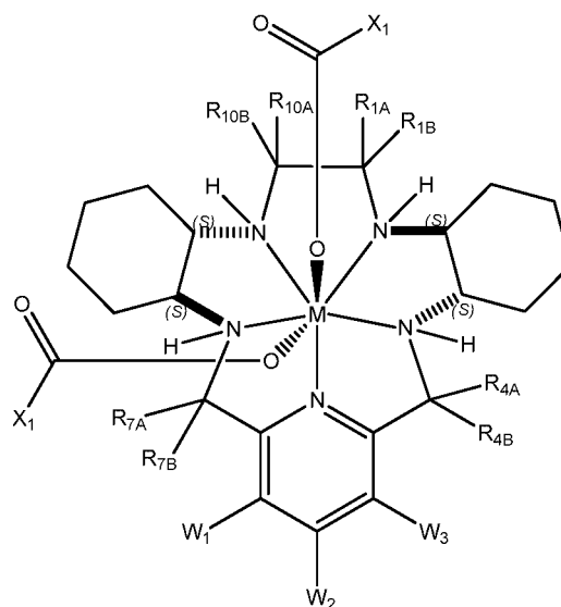
(IC S )
