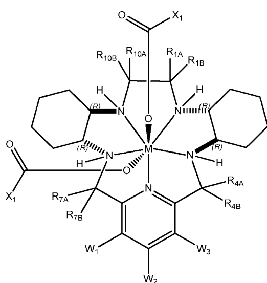
(IC R )
