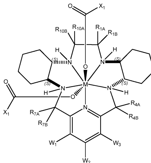
(IC S )
