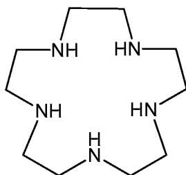
FORMULA A
