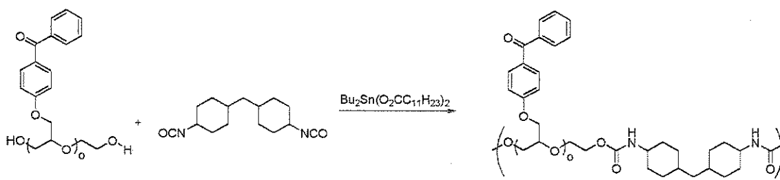
Scheme 2: An exemplified method for preparing a polyurethane-based photoinitiator.
