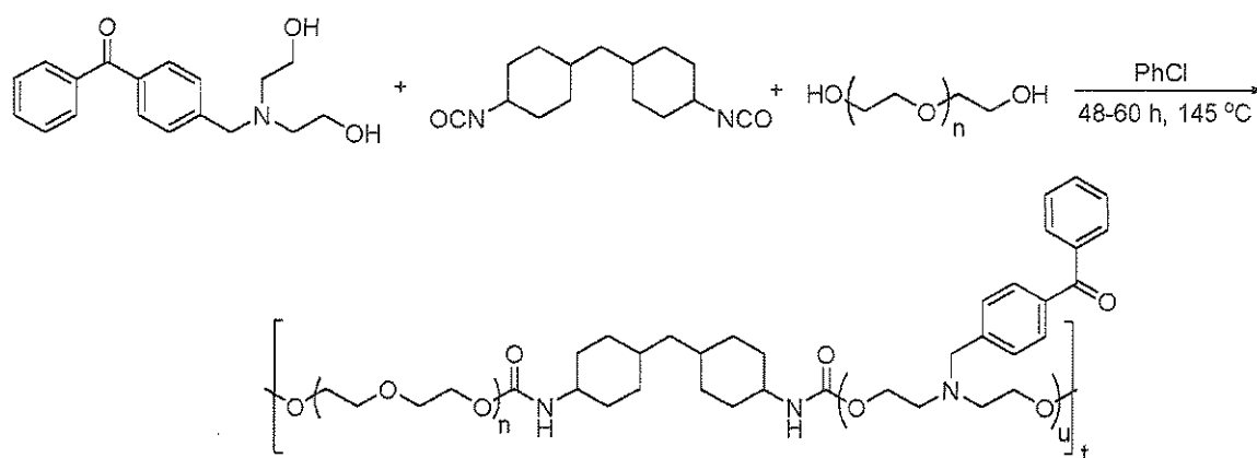
Scheme 4: Synthesis of a polymeric photoinitiator, with a diol derivative of benzophenone, diisocyanate and a polyethylene glycol as the starting materials.
