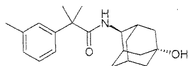
SMP-797
