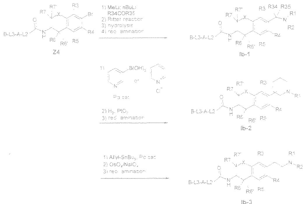
Scheme 2-2
