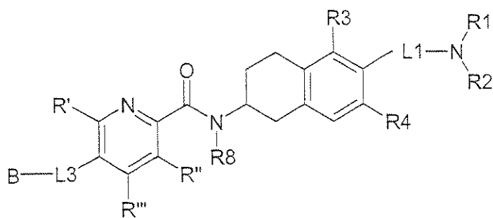
IIa
