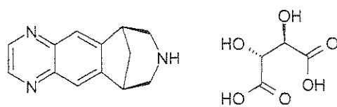
varenicline tartrate
