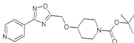
PSN-632408
