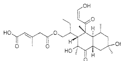
FR-225654
