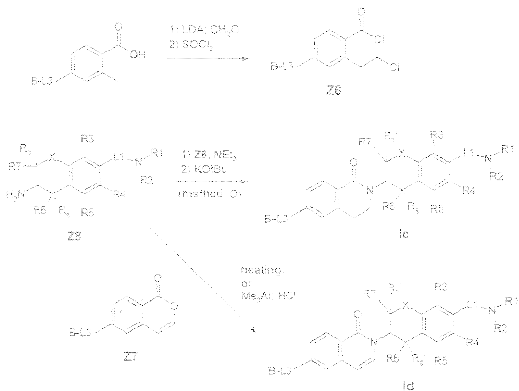
Scheme 3
