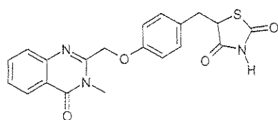
balaglitazone
