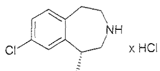
5 lorcaserine hydrochloride
