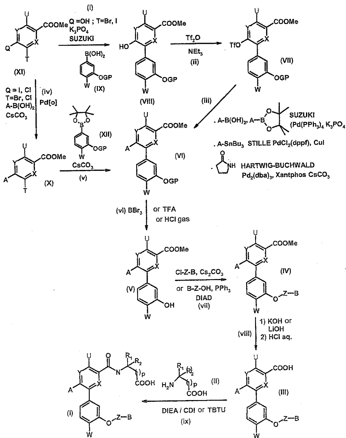
Scheme 1
