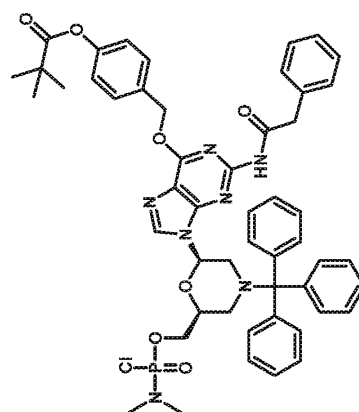
Guanine morpholino monomer
