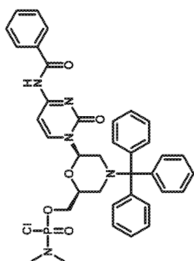
Cytosine morpholino monomer
