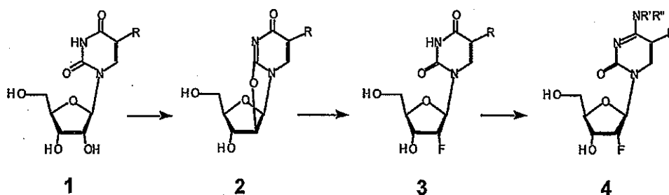
20 Scheme 1. Synthesis of 2'-fluoro-2'-deoxy-uridine and cytidine derivatives.
