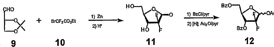
Scheme 3. Preparation of 2,2-difluoro-sugar synthesis for nucleoside synthesis.
