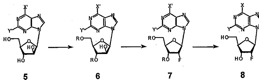
Scheme 2. Synthesis of 2'- \beta -D-ribofuranosylpurine nucleosides.
