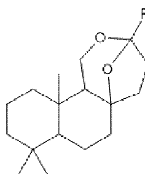
Formula (Ia)
