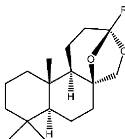
Formula (IV)
