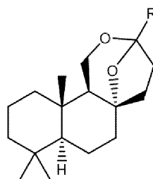
Formula (V)
