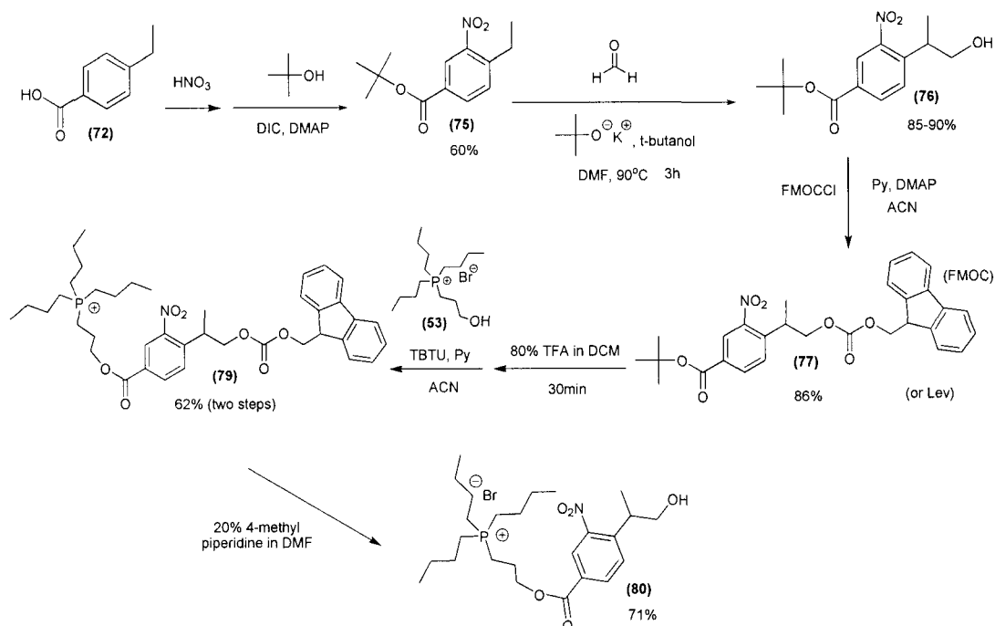
Scheme 15: Synthesis of photolabile ionic tag linker (80)
