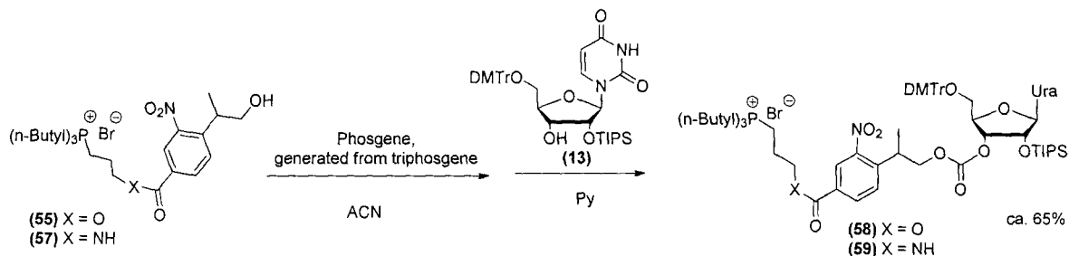
Scheme 31: Conjugation of nucleoside (13) to photolabile ionic tags.
