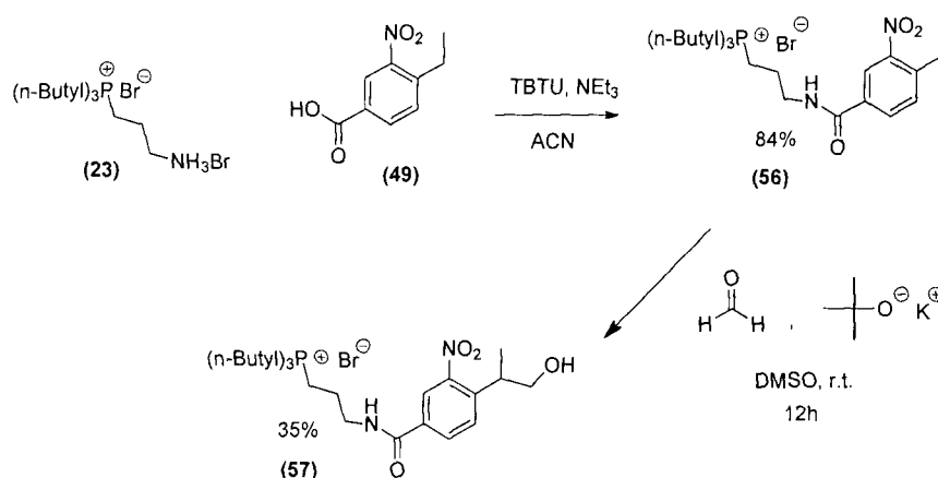
Scheme 30: Short synthesis of photolabile ionic tag (57)
