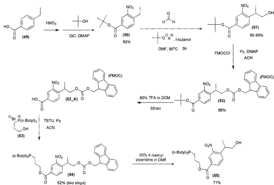
Scheme 29: Synthesis of photolabile ionic tag (55)
