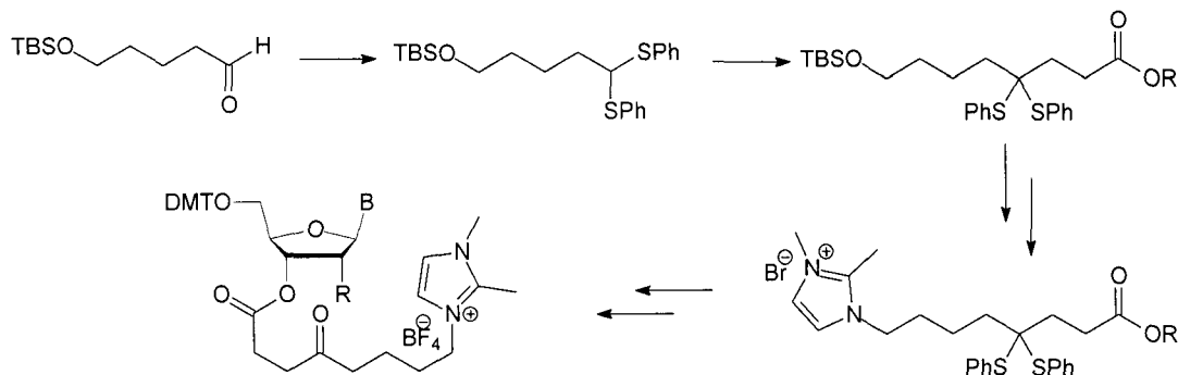
Scheme 14: Dithiane Umpolung approach.
