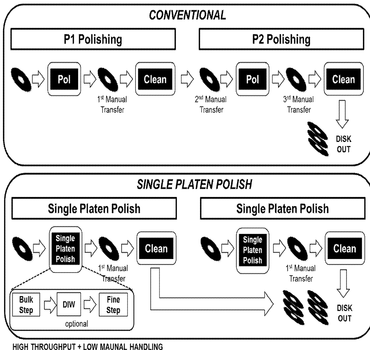
Single-Platen Polish Process versus Conventional 1P+2P (Two-Platen) Polish Process
