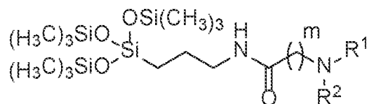
Formula Ia
