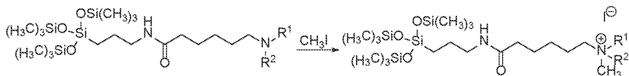
SCHEME 4
