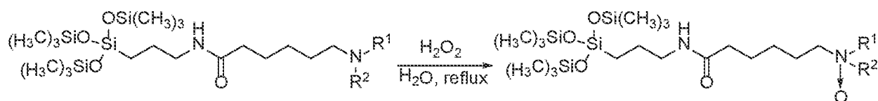
SCHEME 5
