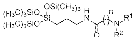
Formula I
