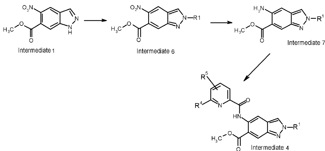
Synthesis Scheme 5
