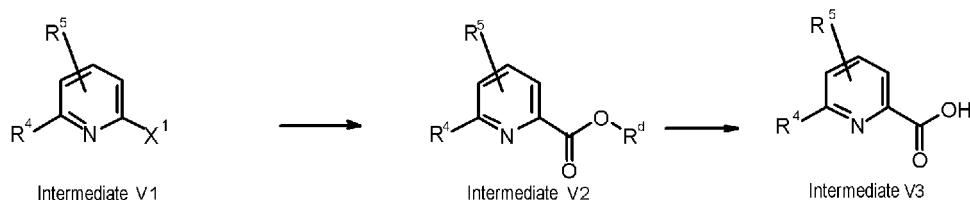
Synthesis Scheme 1
