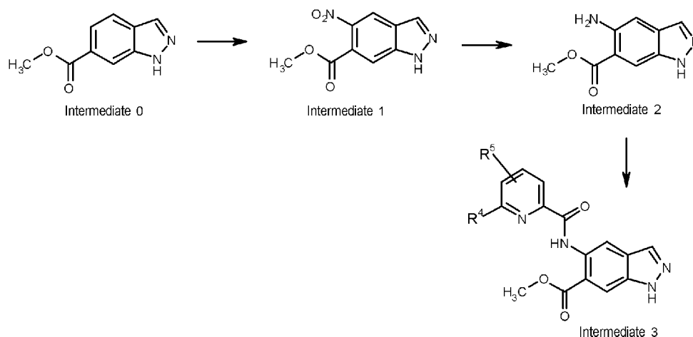
Synthesis Scheme 2
