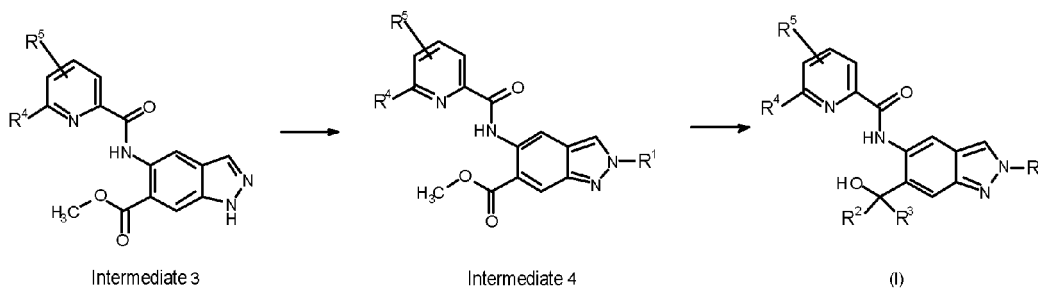
Synthesis Scheme 3
