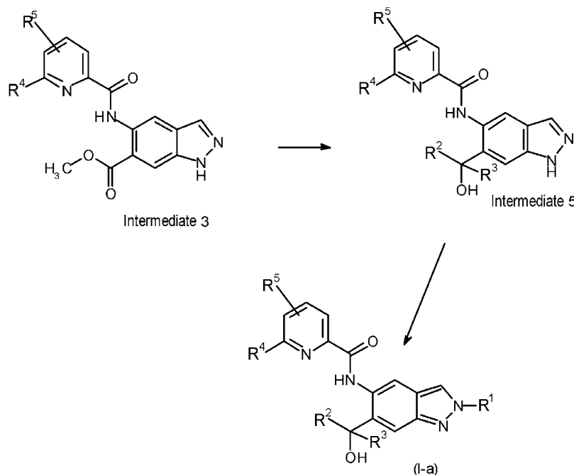
Synthesis Scheme 4
