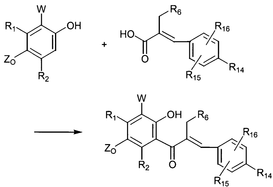
Scheme 6
