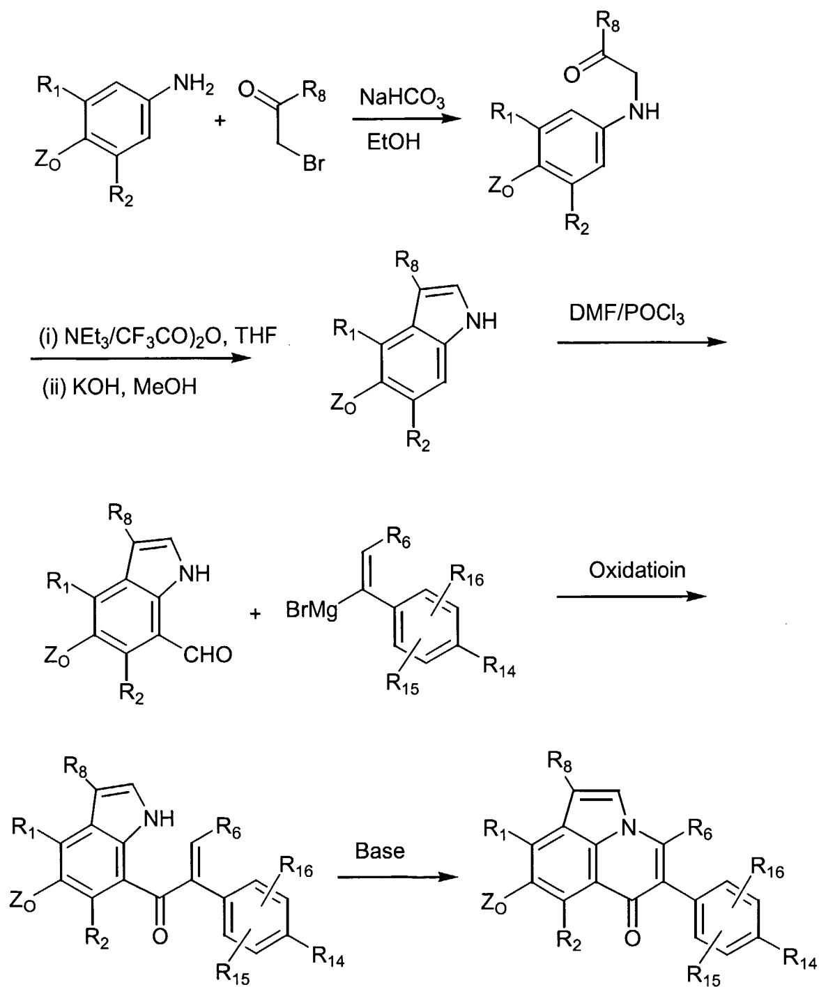
Scheme 7
