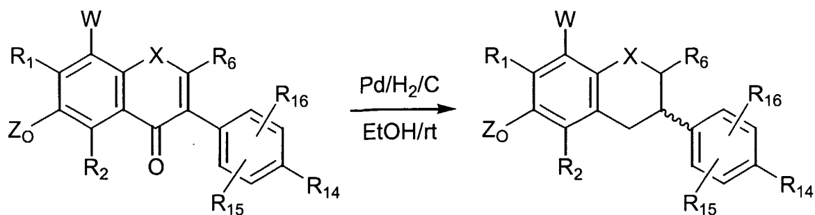
Scheme 3
