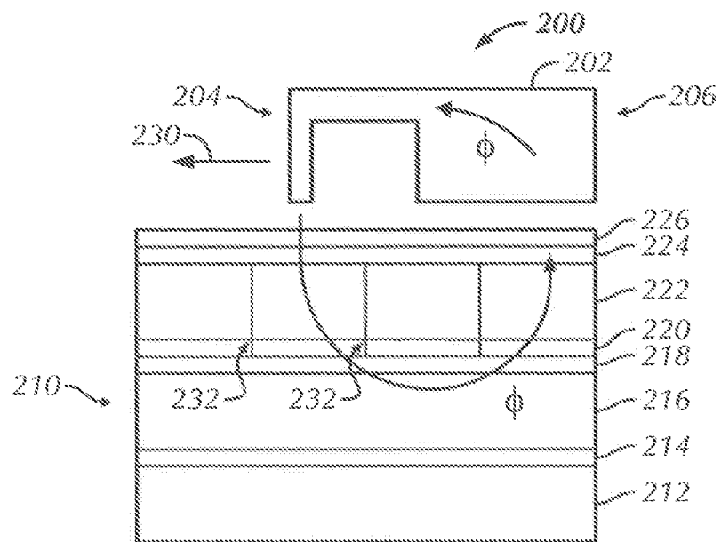
FIG. 2 (Prior Art)
