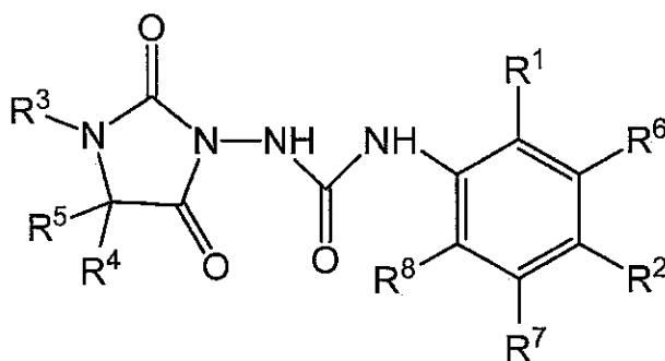
Formula III
