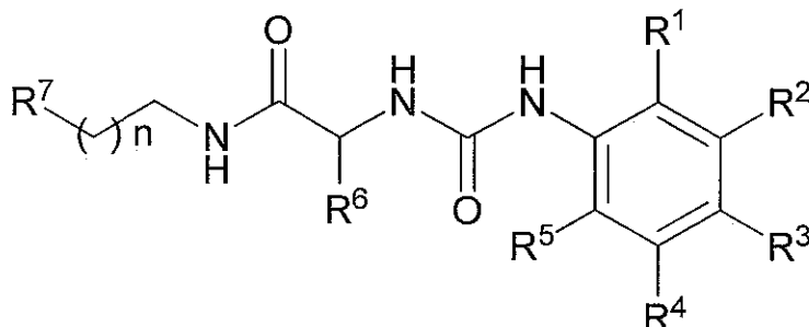
Formula VII
