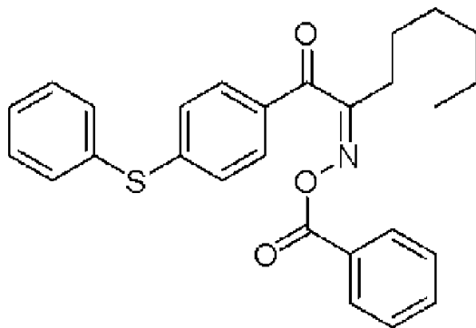
Photopolymerization Initiator 2
