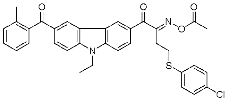
Polymerization Initiator 1
