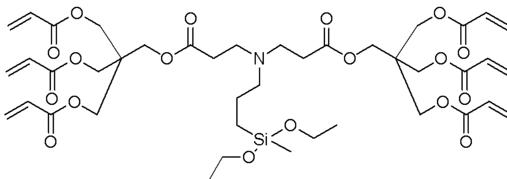
Polymerizable Compound 2
