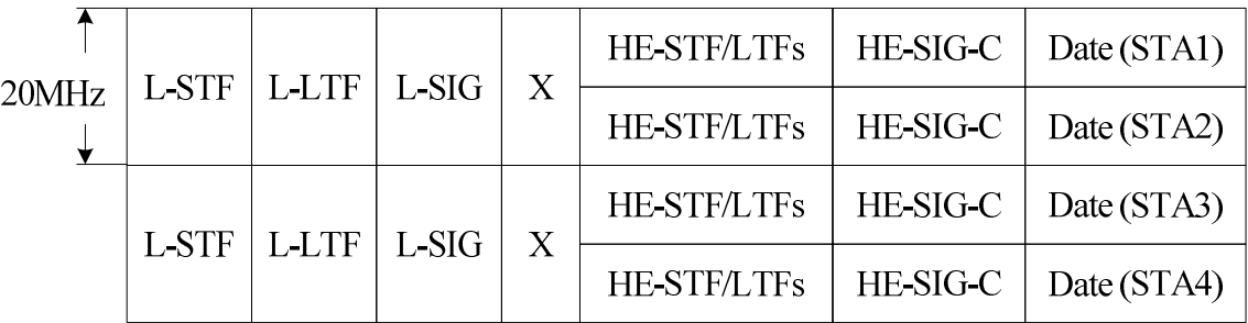
Structure 2: UL MU MIMO, UL OFDMA, DL OFDMA
