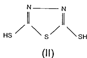
2,5-dimercapto-1,3,4-thiadiazole
