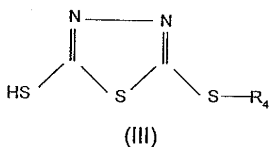
2-mercapto-5-hydrocarbylthio-1,3,4-thiadiazole
