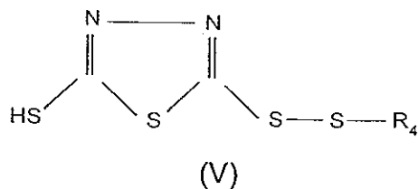
2-mercapto-5-hydrocarbyldithio-1,3,4-thiadiazole
