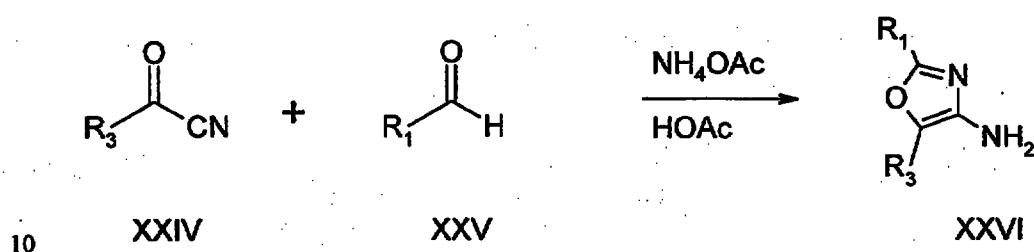
Scheme V
