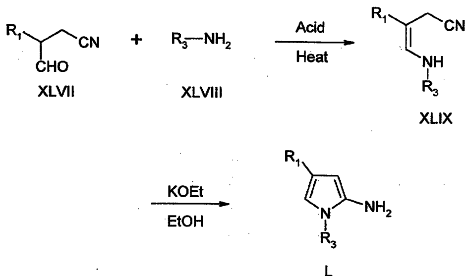
Scheme XII
