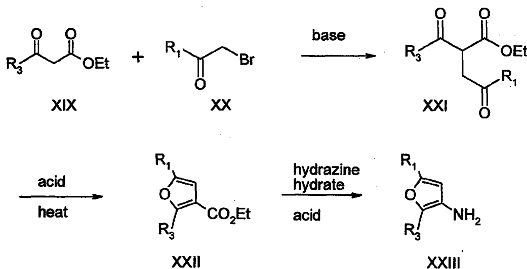
Scheme IV
