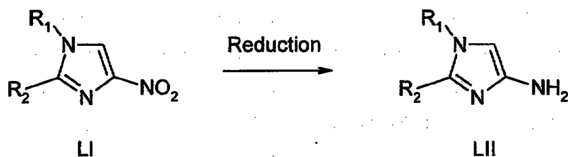
Scheme XIII
