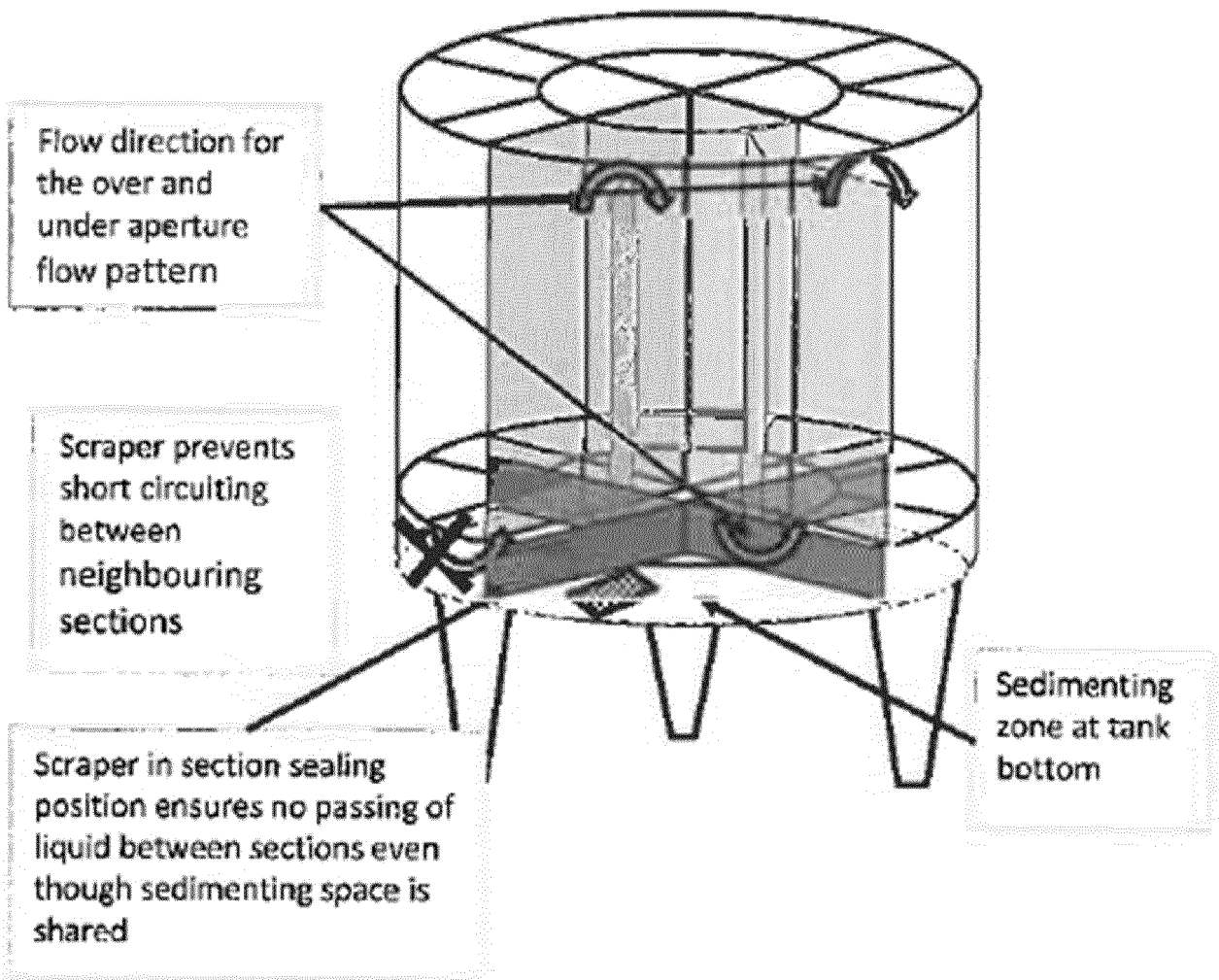
Figure 2. Schematics of the CSTR tank fitted with the FAD insert
