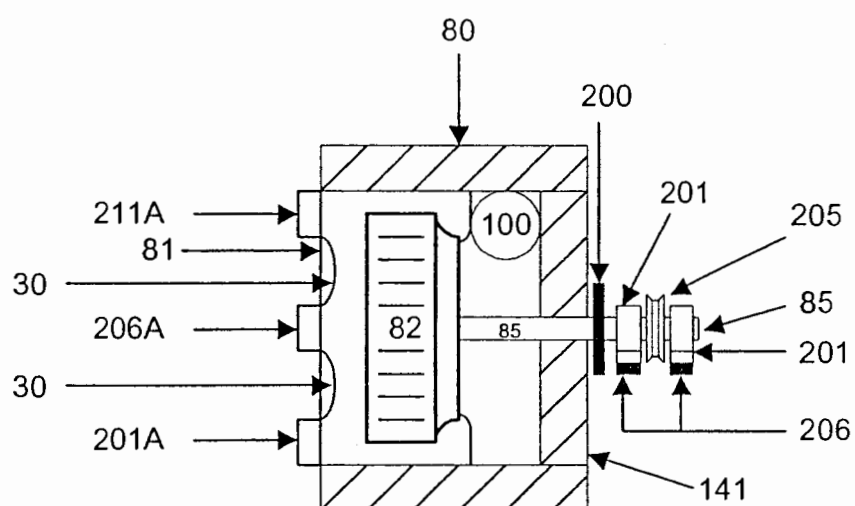
Figure 8 Idle End Fan Sectional View
