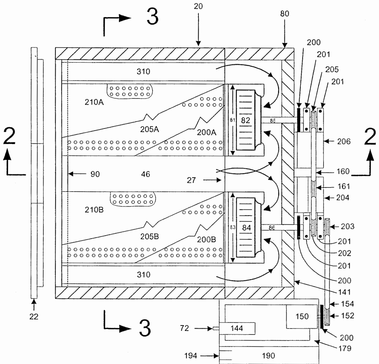
Figure 5 Overhead Sectional View
