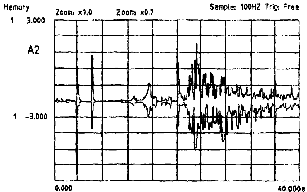
Figure 2 Dynamic response of air-entrained mix - 500 kg/m 3 density
