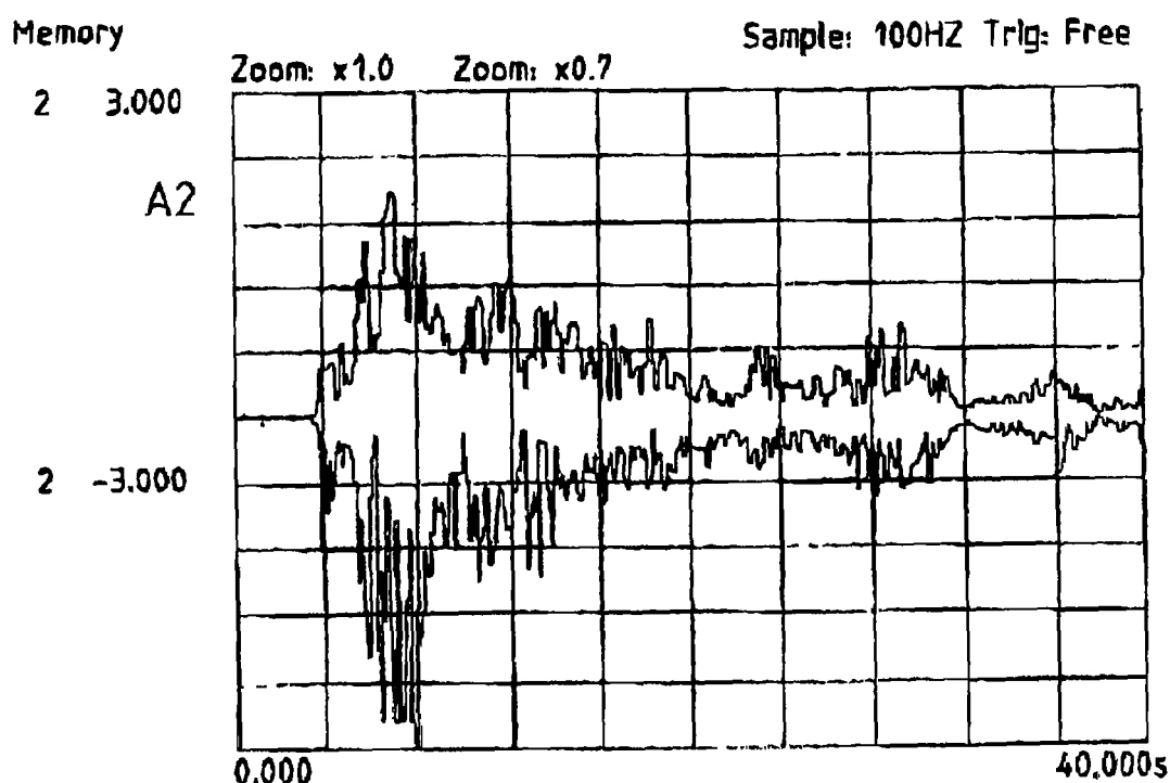
15 Figure 1 Dynamic response of conventional mix - 1100 kg/m 3 density
