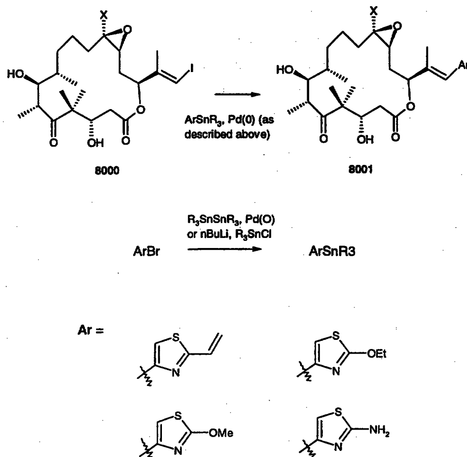
—Scheme 12:
