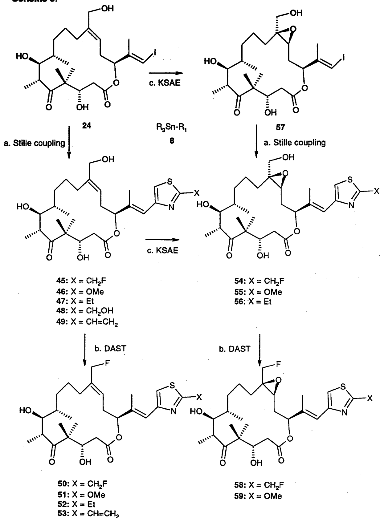
—Scheme 9:
