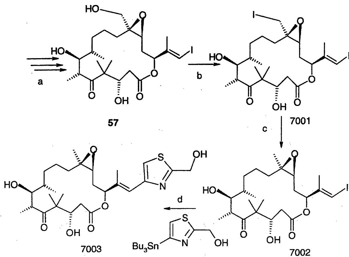
—Scheme 11:
