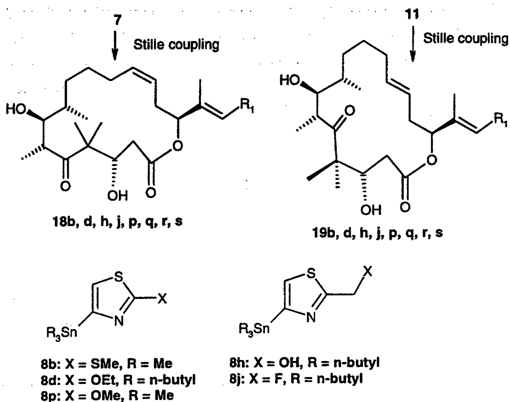
—Scheme 3:
