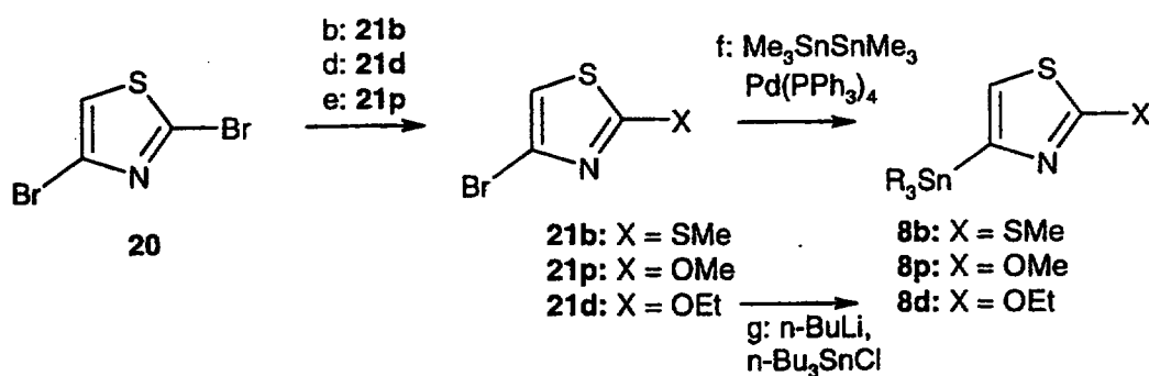
—Scheme 4:
