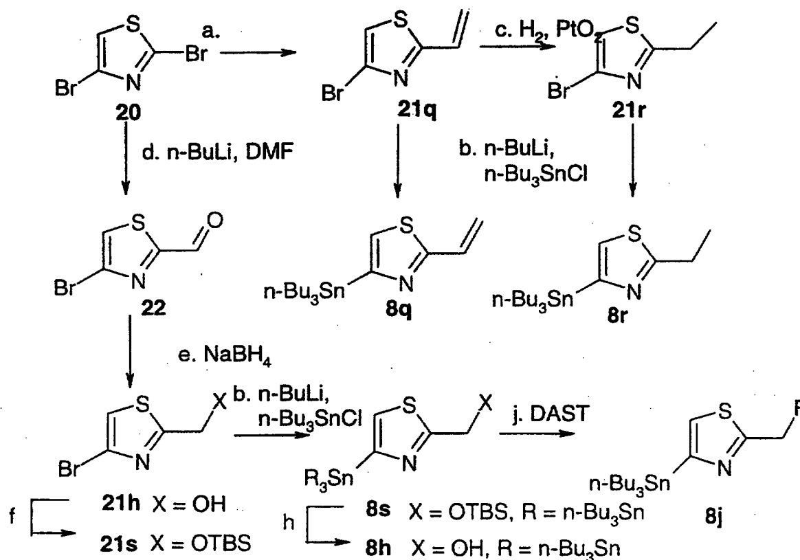
—Scheme 5:
