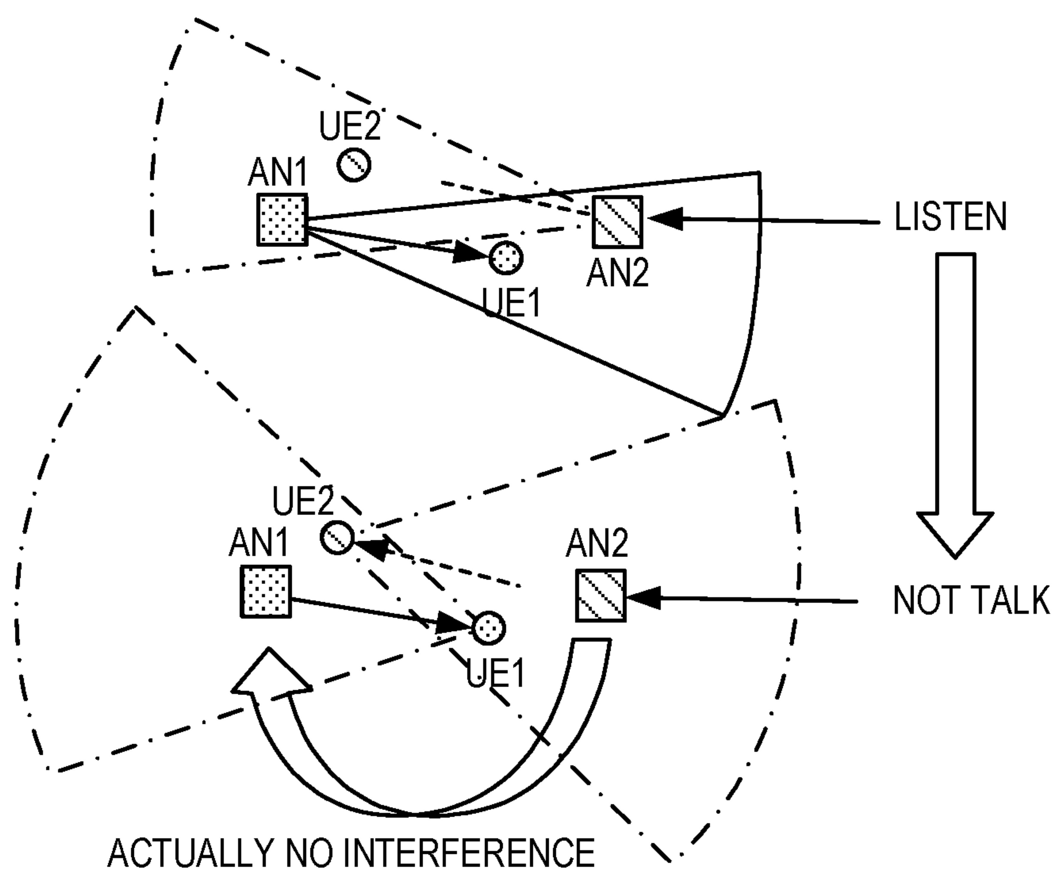
B) EXPOSED NODE PROBLEM
