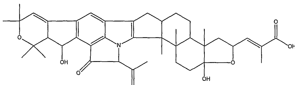
29,30-dihydro-20,30-oxa-nodulisporic acid (compound B)
