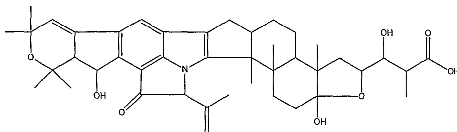
5 31-hydroxy-20,30-oxa-29,30,31,32-tetrahydro-nodulisporic acid (compound C)
