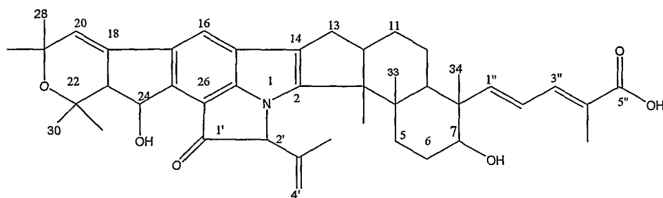
29,30-dihydro-20,30-oxa-nodulisporic acid (compound B)
