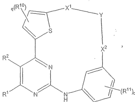
Formula (III)
