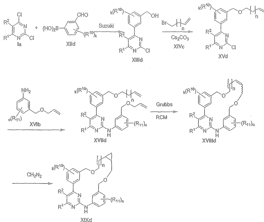
Scheme 3
