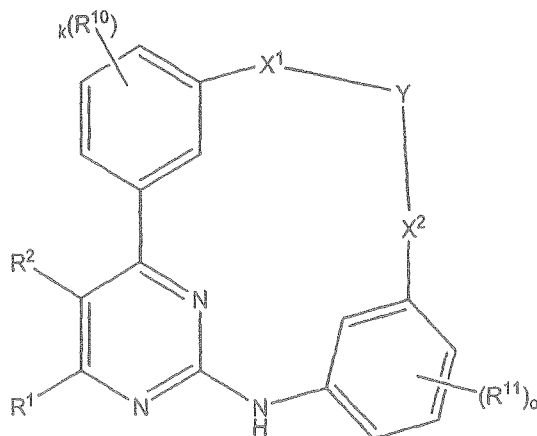
Formula (II)
