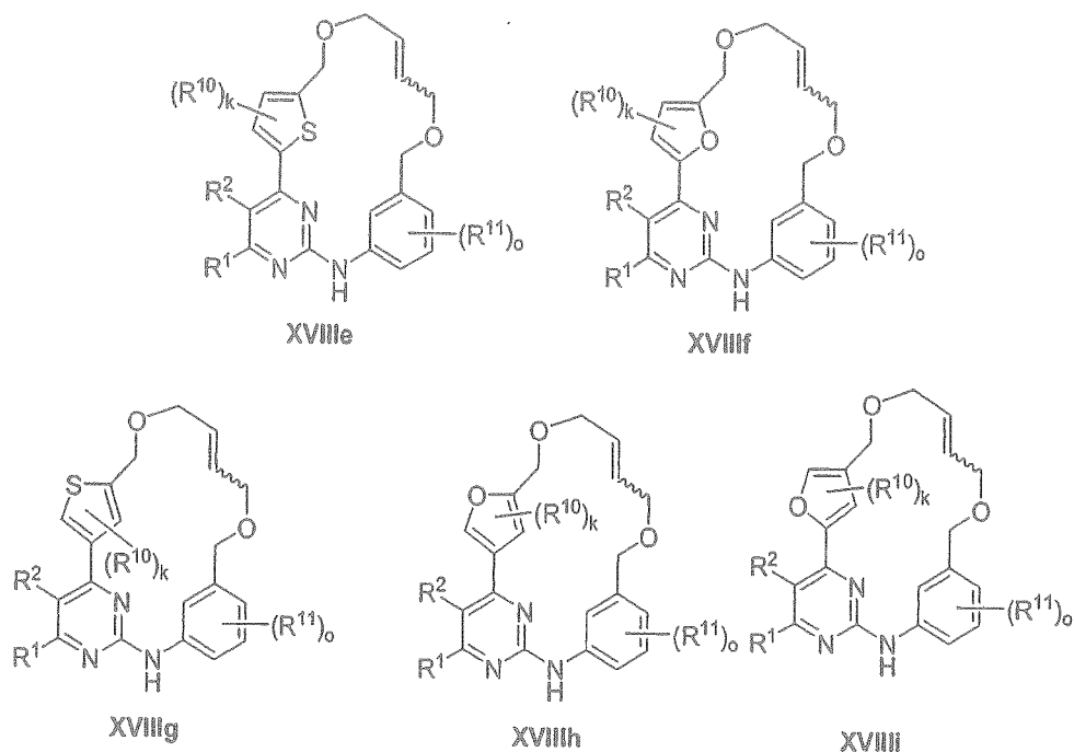
Scheme 4
