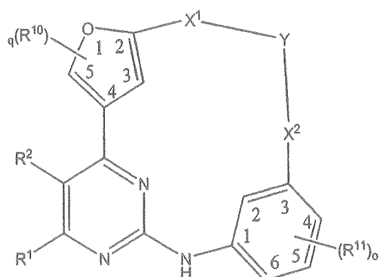
Formula (VI)
