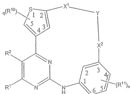
Formula (IV)
