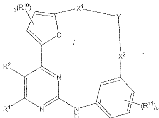
Formula (V)
