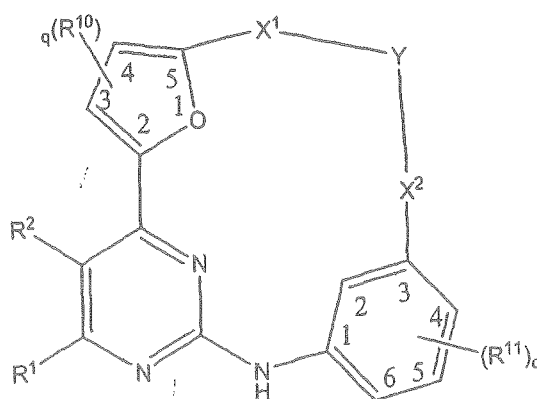
Formula (V)
