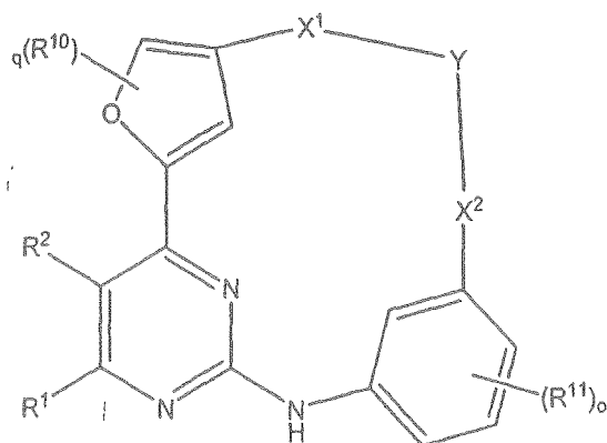
Formula (VII)
