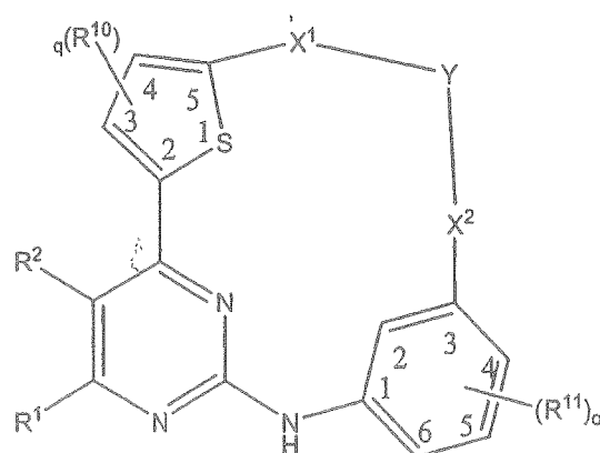
Formula (III)
