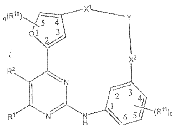
Formula (VII)
